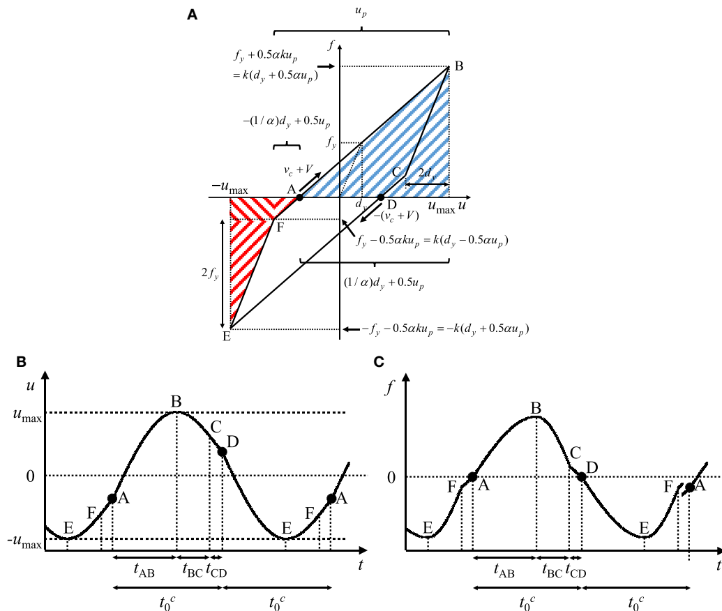
FIGURE 6 | Derivation of maximum deformation under critical multi impulse based on energy approach: (A) restoring-force deformation relation; (B) displacement time history; (C) restoring-force time history (CASE 2: V/V_y \geq -2 + 2\sqrt{1/\alpha} ).
