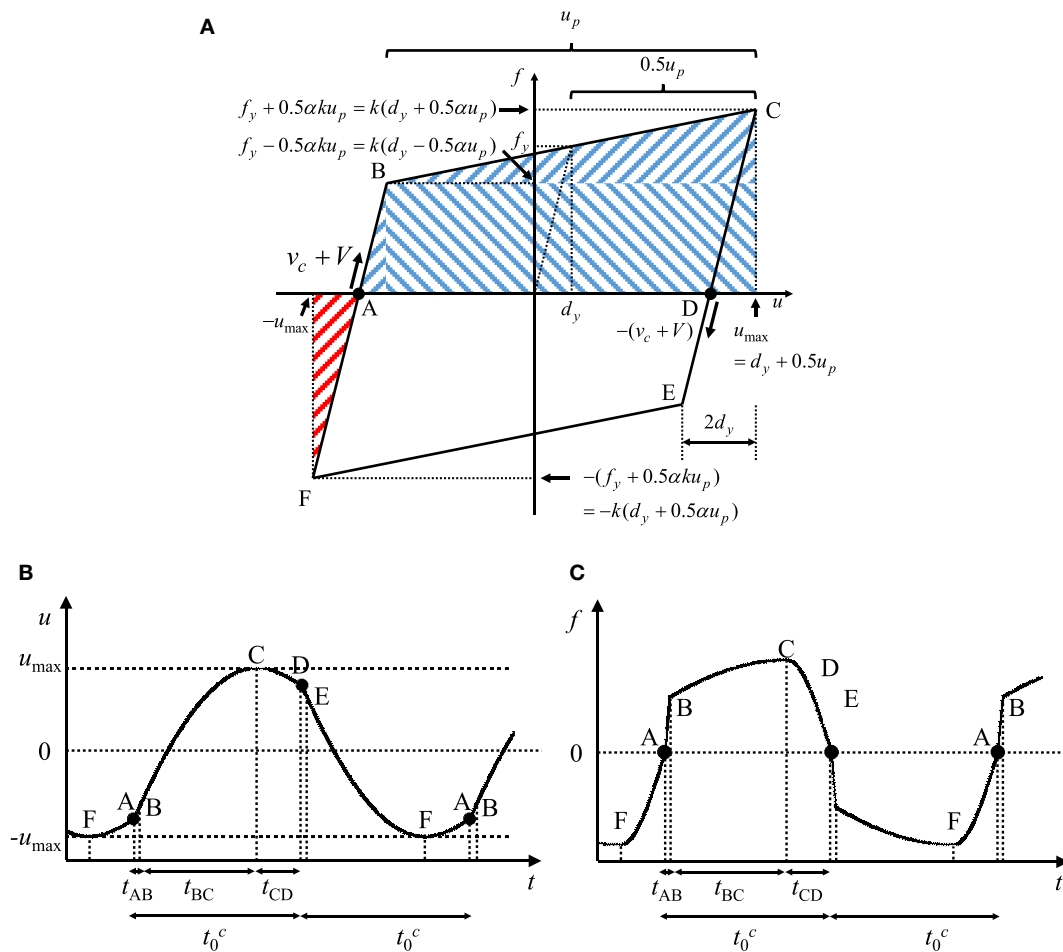
FIGURE 4 | Derivation of maximum deformation under critical multi impulse based on energy approach: (A) restoring-force deformation relation; (B) displacement time history; (C) restoring-force time history (CASE 1: V/V_y < -2 + 2\sqrt{1/\alpha} ).
