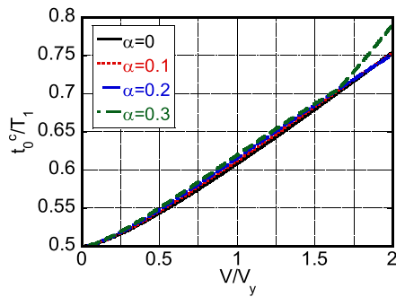
FIGURE 8 | Critical impulse timing t_0^c/T_1 with respect to input level V/V_y for various post-yield stiffness ratios \alpha .
