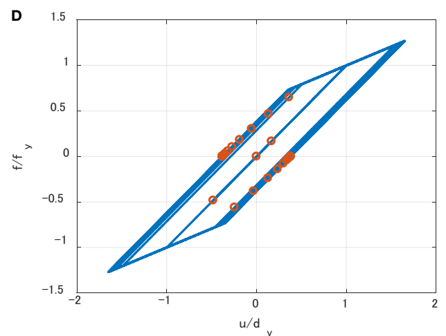
restoring force-deformation
