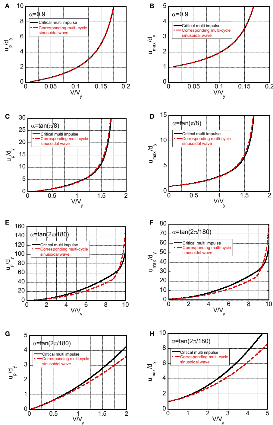
FIGURE 12 | Comparison of plastic deformation and maximum deformation between critical multi impulse and corresponding multi-cycle sinusoidal wave: (A,B) \alpha = 0.9 , (C,D) \alpha = \tan(\pi/8) = 0.414 , (E,F,G,H) \alpha = \tan(2\pi/180) = 0.0349 [(G,H) are magnified ones of (E,F)].
