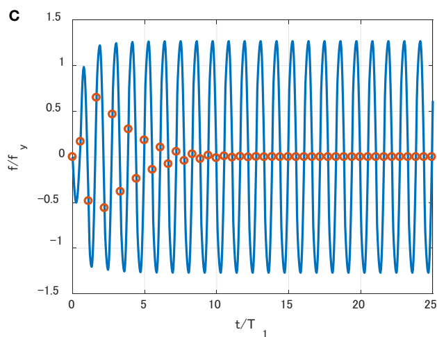
restoring force
