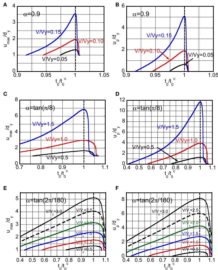
FIGURE 13 | Maximum deformation and plastic deformation amplitude with respect to timing of multi impulse for various input levels: (A,B) \alpha = 0.9 , (C,D) \alpha = \tan(\pi/8) = 0.414 , (E,F) \alpha = \tan(2\pi/180) = 0.0349 .
