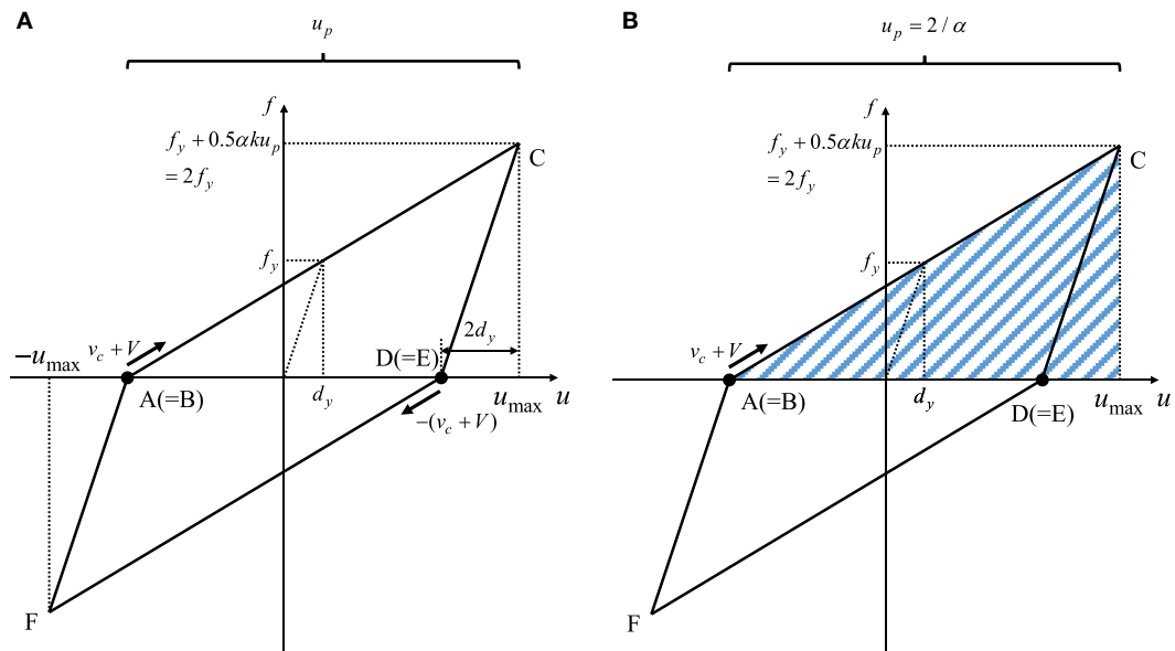
FIGURE 5 | Restoring-force deformation relation in the boundary case between CASE 1 and CASE 2: (A) acting points of each impulse; (B) sum of hysteretic and elastic strain energy after each impulse.
