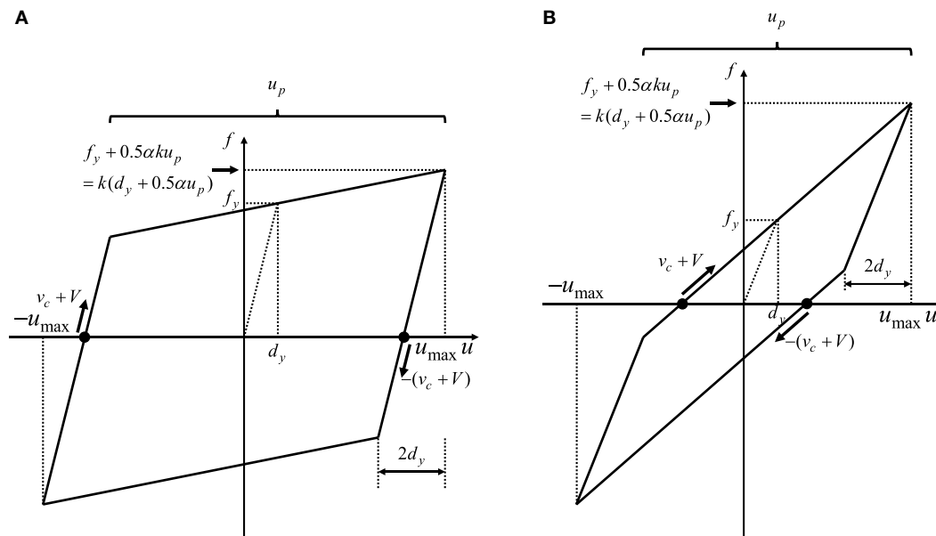
FIGURE 3 | Restoring-force deformation relation under critical multi impulse: (A) CASE 1 ( u_p/d_y \leq 2/\alpha ): impulse in unloading process; (B) CASE 2 ( u_p/d_y > 2/\alpha ): impulse in loading process.
