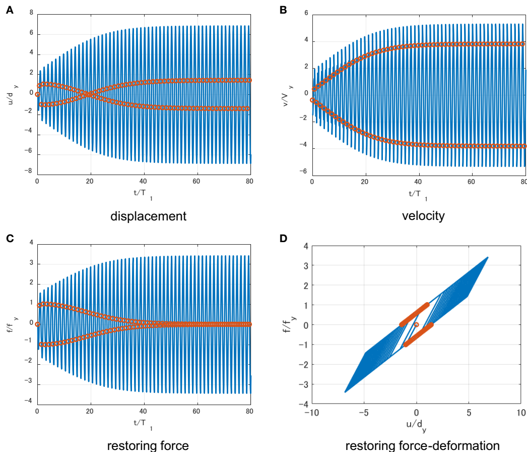
FIGURE 11 | Response under multi impulse with time interval t_0^c for V/V_y = 1.5 and \alpha = \tan(\pi/8) = 0.414 (impulse timing is the critical one obtained by steady-state assumption): (A) displacement, (B) velocity, (C) restoring force, and (D) restoring-force deformation relation.
