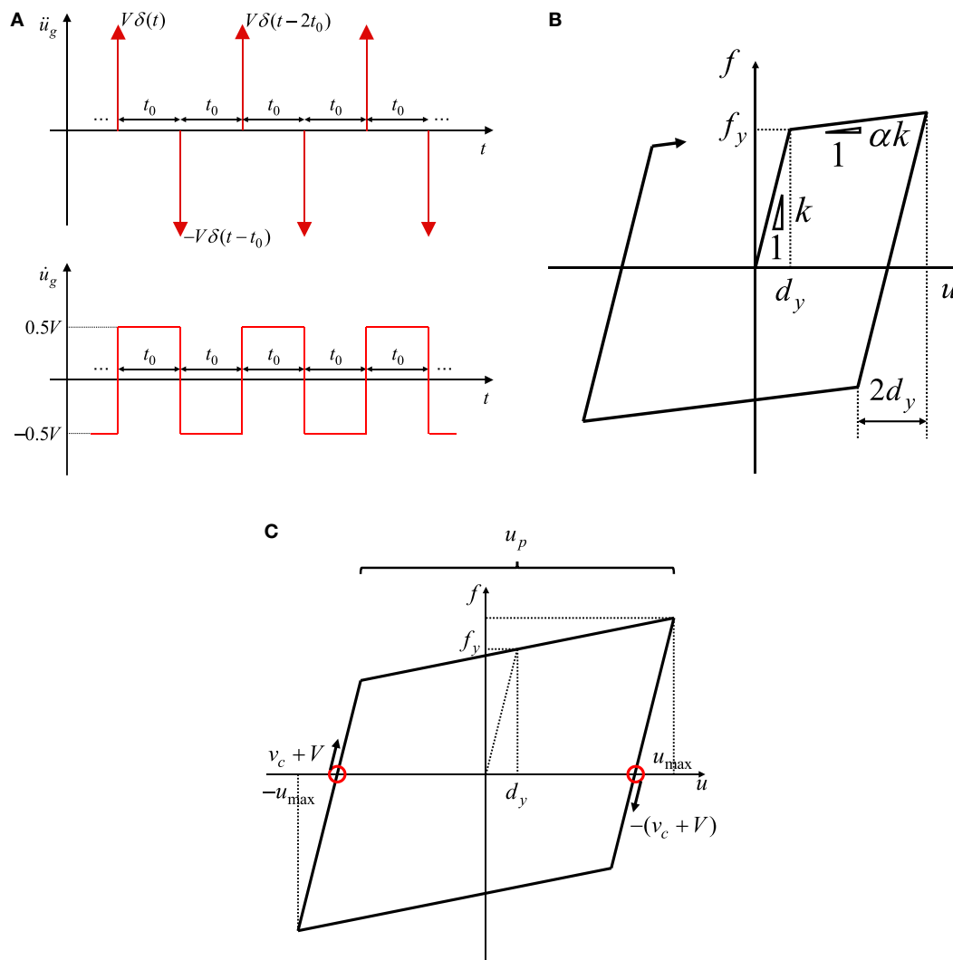
FIGURE 2 | Impulse input and bilinear hysteretic restoring-force deformation characteristic: (A) multi impulse with equal time interval t_0 , (B) bilinear hysteretic restoring-force characteristic, (C) steady-state loop under critical multi impulse.
