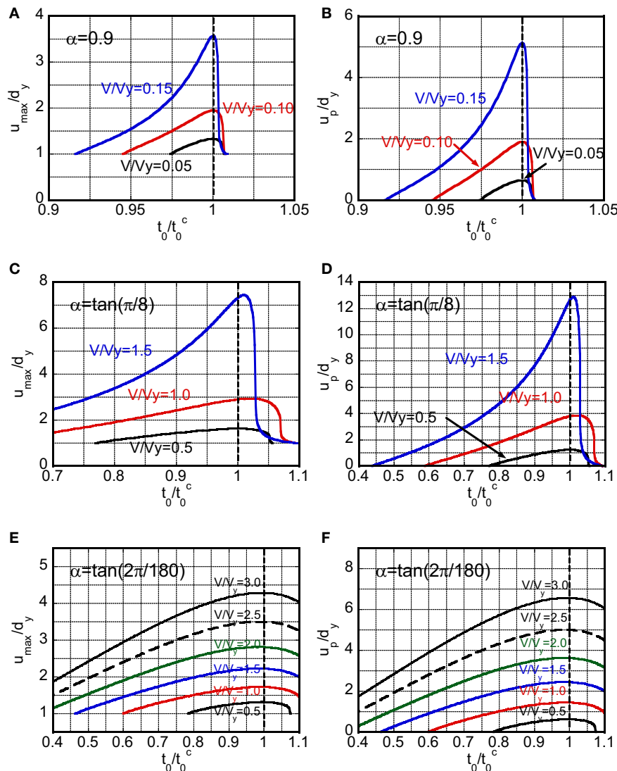
FIGURE 14 | Maximum deformation and plastic deformation amplitude with respect to period of corresponding sinusoidal wave for various input levels: (A,B) \alpha = 0.9 , (C,D) \alpha = \tan(\pi/8) = 0.414 , (E,F) \alpha = \tan(2\pi/180) = 0.0349 .
