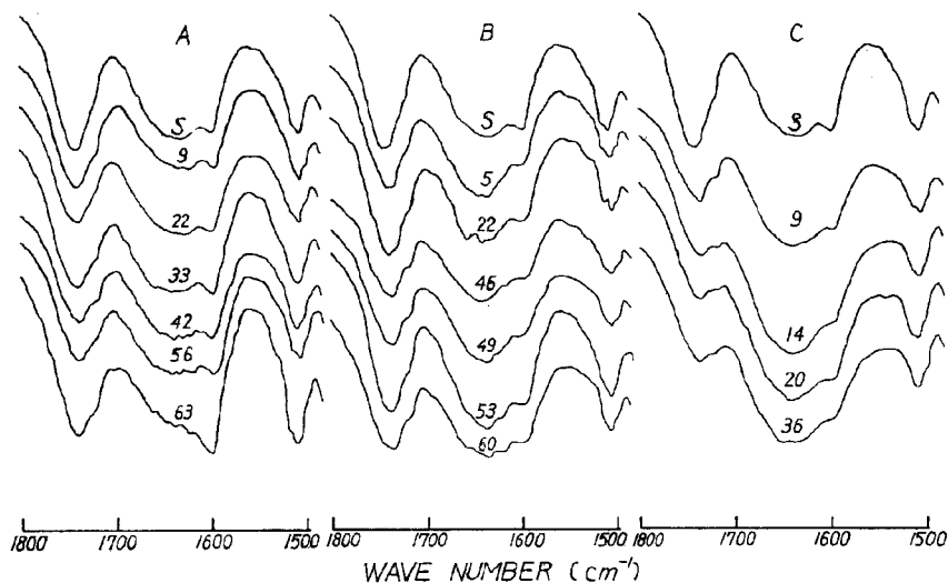
Fig. 1. Infrared spectra of BUNA wood decayed by C. palustris (A), C. versicolor (B) and C. globosum (C) in the 1800\text{--}1500\text{ cm}^{-1} region. S: sound, figures on spectra: percents weight loss of decay wood blocks.
