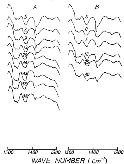
Fig. 4. Infrared spectra of SUGI wood decayed by C. palustris (A) and C. versicolor (B) in the 1500-1300 \text{cm}^{-1} region. S: sound, figures on spectra: percent weight loss of decayed wood blocks.
