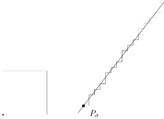
Figure 2. (e_1, 1^*) + (e_2, 2^*) and \sigma^*((e_1, 1^*) + (e_2, 2^*)) for x = [0, 4, \overline{4, 2}]
