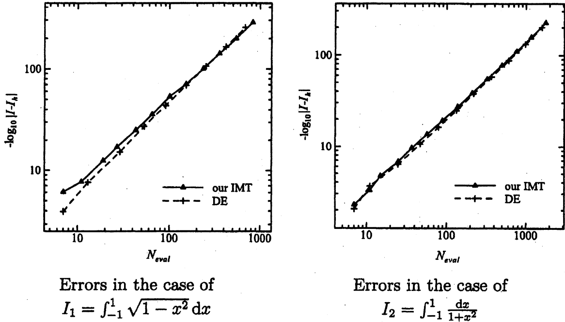
Fig. 1: Comparison between our formula and the DE formula for I_1 and I_2
