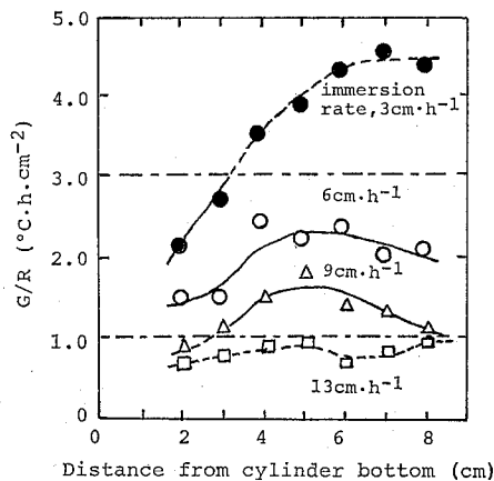
Fig. 7. Ratio of temperature gradient ( G ) to freezing rate ( R ) versus distance from cylinder bottom during unidirectional freezing of gel derived from \text{Al}_2\text{O}_3 sol C2.
