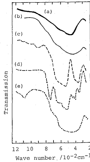
Fig. 12. IR spectra of freeze-formed zirconia fibers as-dried at 25^{\circ}\text{C} (a) and heated at 290^{\circ}\text{C} (b), \text{CaZrO}_3 (c), monoclinic \text{ZrO}_2 (d) and (\text{ZrO}_2)_{0.8}(\text{Y}_2\text{O}_3)_{0.2} (e) crystals.
