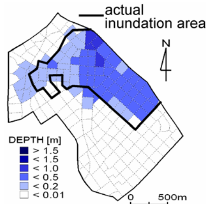
Fig.4.7 Maximum inundation depth on the ground
