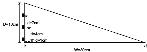
Fig.5.2 Model barrier and pressure measurement
