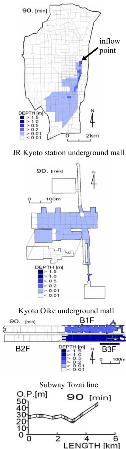
Fig.4.13 Computed inundation water depth distributions at 90min.
