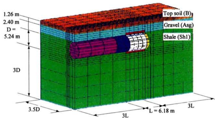
Figure 3.34 Simulation mesh of the tunneling project
