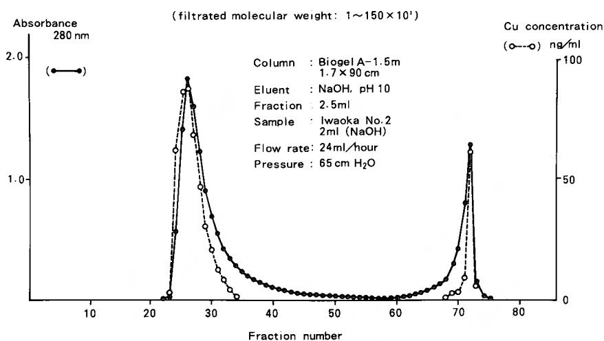
Fig. 33. Gel filtration of black components (filtrated molecular weight: 1\sim150\times10^4 )
