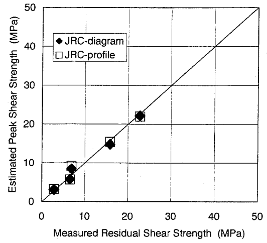
(b) Residual shear strength (1st shear test)
