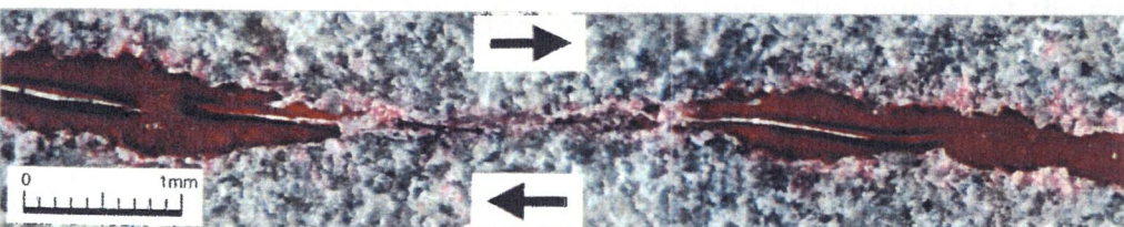
(e) Shear displacement of 2mm
