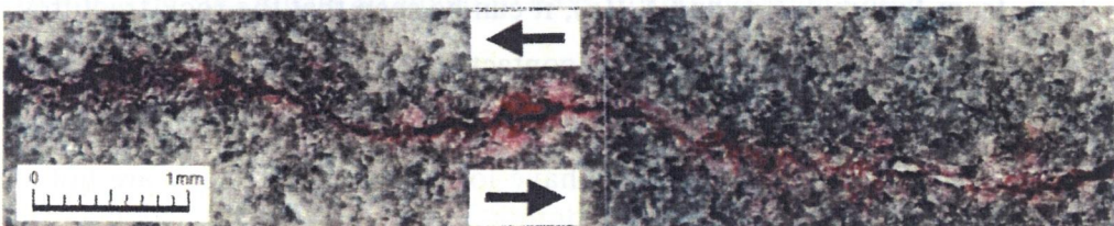
(c) Just after the peak shear strength
