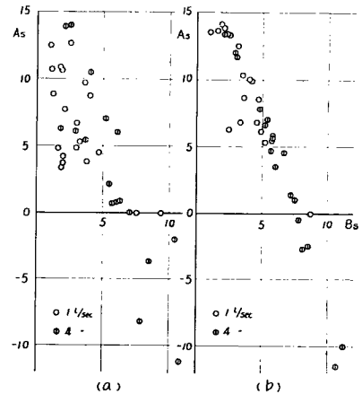
Fig. 10 Values of A_s and B_s as using Eq. (15)
