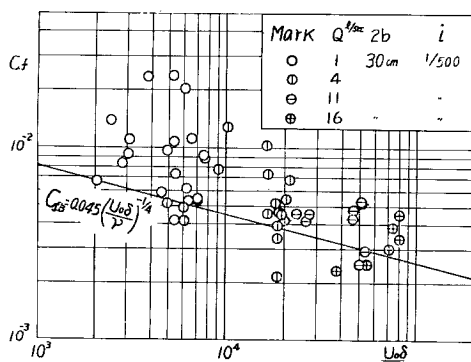
Fig. 4 Relation between C_f and u_0 \delta / \nu
