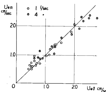
Fig. 5 Relation between u_* R , u_* \delta and u_* B
