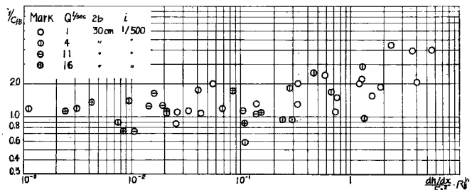
Fig. 11 Relation between C_f/C_{fB} and \frac{dh/dx}{F_\delta^2} \cdot R\delta^{1/4}
