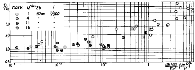
Fig. 12 Relation between f/f_B and \frac{dh/dx}{F_R^2} \left( \frac{u_m R}{\nu} \right)^{1/4}
