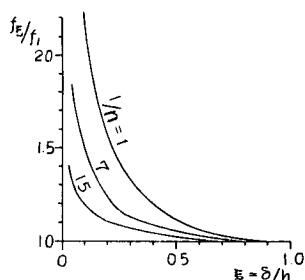
Fig. 6 Relation between f_\xi/f_1 and \xi
