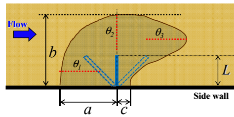
Fig. 6 Sketch of scour hole dimension parameters
