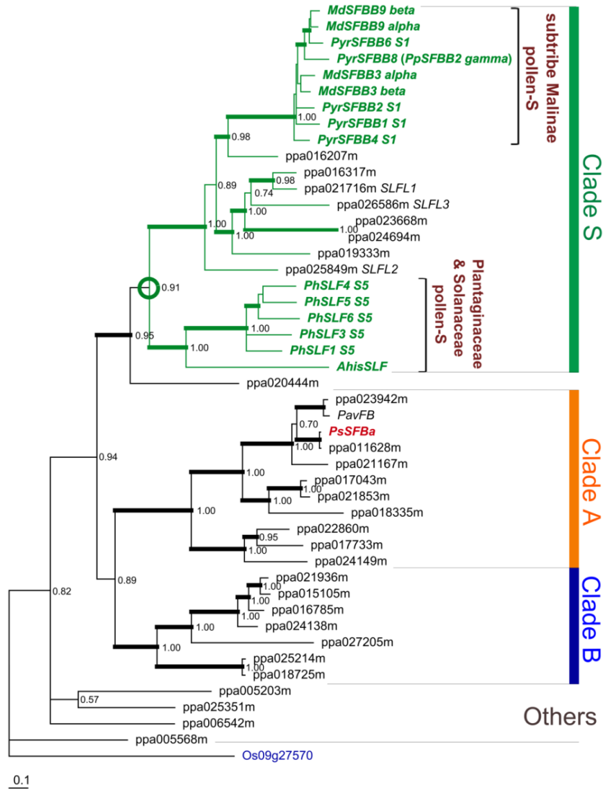
Fig. 1.1 Phylogenetic tree of SFB/SLFL -like F-box genes from the Prunus persica genome. Bayesian MCMC phylogenetic tree for SFB/SLFL -like F-box genes from P. persica (prefixes of “ppa”) along with pollen S F-box genes from Antirrhinum , Petunia and subtribe Malinae. The position of the most recent common ancestor of the original pollen S is indicated by a green circle. The pollen S F-box gene in Prunus , SFB , is highlighted in red. Thick branches indicate clades with strong statistical support (Bayesian posterior probability > 0.95).
