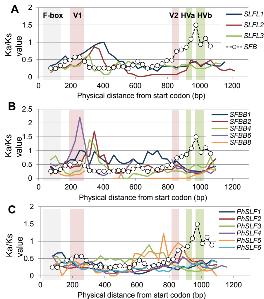
Fig. 1.7 Selective pressure on SFB/SLFL -like F-box genes in Prunus , Pyrus and Petunia . Mean pairwise Ka/Ks ratios between alleles from (A) Prunus SFB and three SLFLs located around the Prunus S locus, (B) Prunus SFB and five SFBBs from Pyrus and (C) Prunus SFB and six SLFs from Petunia . The F-box region, two variable regions (V1 and V2), and two hypervariable regions (HV a and HV b ) of the SFB gene are colored in gray, red and green, respectively. SFB data is shown by the dotted line with white circles.
