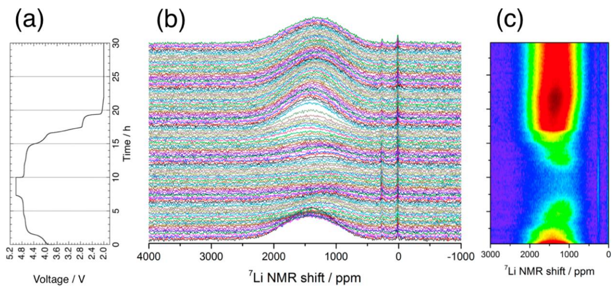
Figure. 5. In situ ^7\text{Li} static NMR spectra of \text{Li} // \text{LiNi}_{0.4}\text{Mn}_{1.6}\text{O}_4 ( Fd\bar{3}m structure) cell. (a) Charge-discharge profile (0.1C rate) as a function of time, (b) stacked, and (c) contour plots of in situ ^7\text{Li} spectra.
