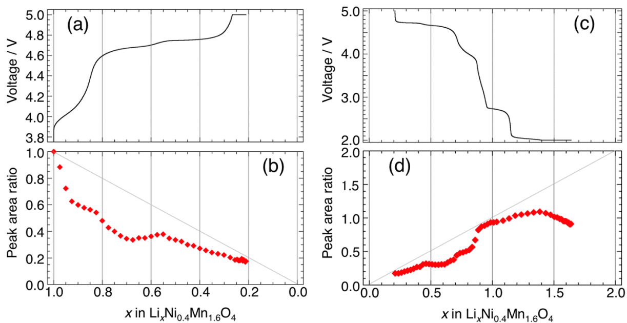
Figure 7. (a) Charging profile up to 5.0 V and (b) peak area extracted from in situ ^7\text{Li} spectra of the \text{LiNi}_{0.4}\text{Mn}_{1.6}\text{O}_4 electrode. (c) Discharging profile down to 2.0 V and (d) peak area variation.
