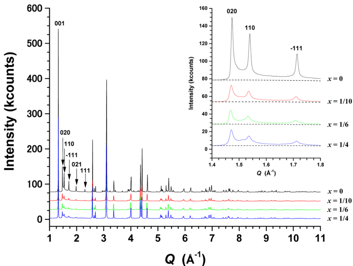
Figure 3. Synchrotron diffraction patterns of \text{Li}_2(\text{Ni}_x\text{Mn}_{1-x})\text{O}_{3(-\delta)} ( x = 0, 1/10, 1/6, \text{ and } 1/4 ). The arrows indicate the positions of the 020, 110, \bar{1}11 , 021, and 111 superstructure reflections. The insets show magnified images of the low-angle parts; fairly intense diffuse peaks from the stacking faults can be seen, especially at the bottoms of the 020, 110, and \bar{1}11 superstructure reflections (the background profiles are represented by the broken lines).
