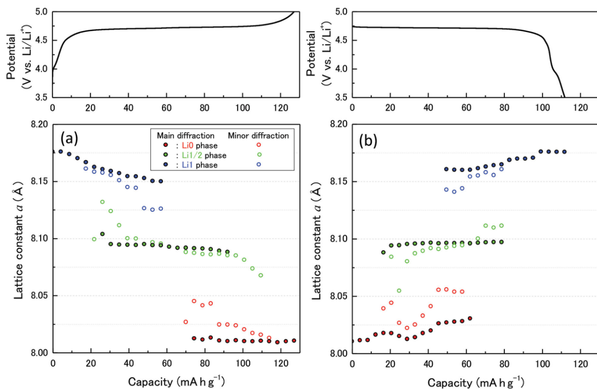
Figure 4. Variation of lattice constants of a \text{LiNi}_{0.5}\text{Mn}_{1.5}\text{O}_4 electrode obtained from peak centers of partial diffraction profiles with the corresponding electrode potential profiles during (a) charging and (b) discharging at rate of 1 C.
