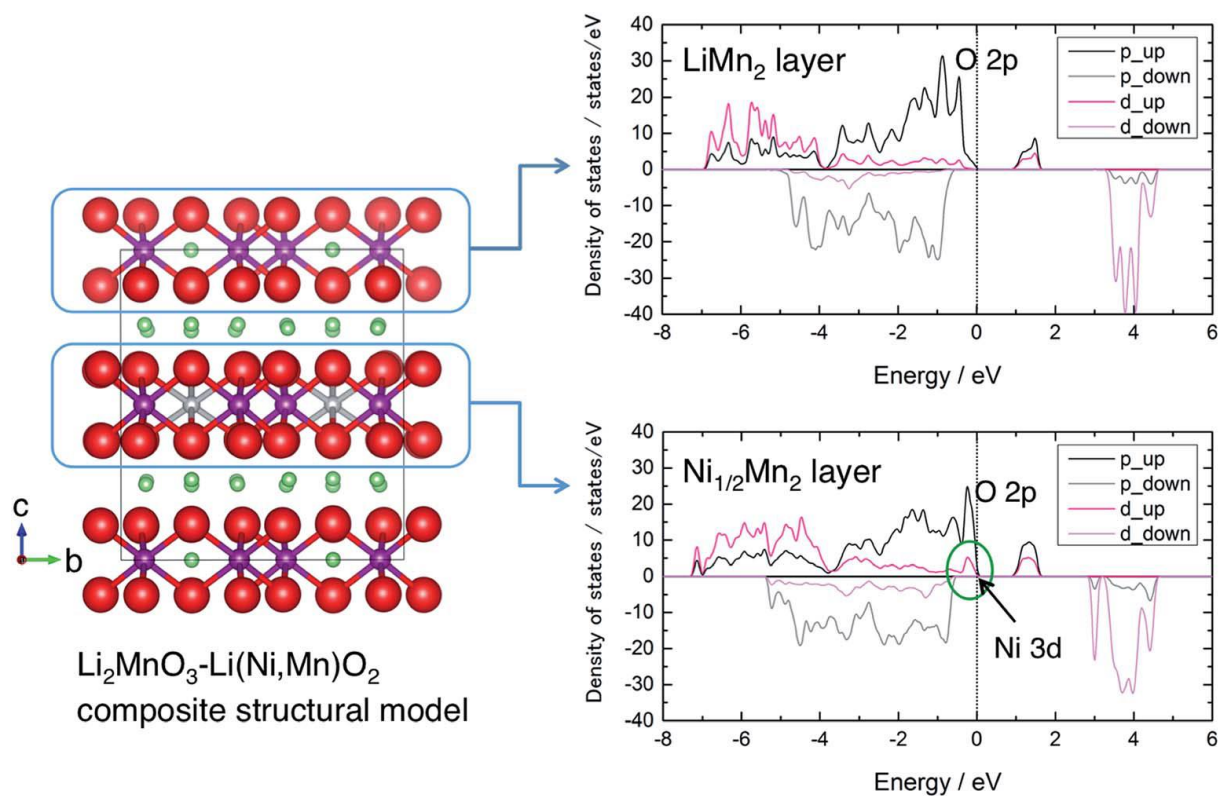
Figure 13. A \text{Li}_2\text{MnO}_3\text{-Li(Ni,Mn)O}_2 -like composite structural model and calculated density of states of the \text{LiMn}_2 layer ( \text{Li}_2\text{MnO}_3 -like domain) and \text{Ni}_{1/2}\text{Mn}_2 layer ( \text{Li(Ni,Mn)O}_2 -like domain). O: red sphere, Mn: purple sphere, Ni: gray sphere, and Li: green sphere. The p and d components are almost exclusively dominated by O 2p and Ni/Mn 3d states, respectively. The “up” and “down” denote majority and minority spin states, respectively.
