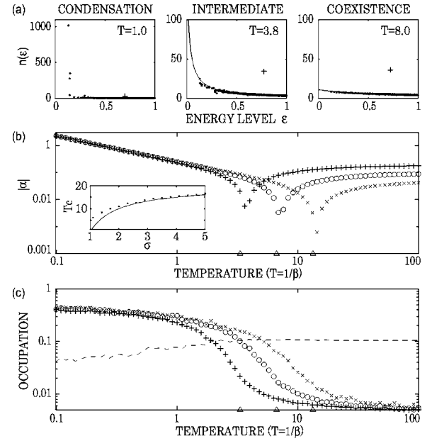
FIG. 1. (a) Normalized cumulative gain n_i(\epsilon_i) for m=5 and T < T_c (left), T \approx T_c (center), and T > T_c (right). The solid line is the Bose distribution with \alpha from Eq. (11). The plus sign indicates a pioneer. Plots of the last ten entrants were excluded. (b) Numerical calculation of |\alpha| with \alpha from Eq. (11), averaged over 500 trials. Symbols +, \circ , and \times indicate m=5 , 10, and 20. Change in the sign of \alpha indicates the transition. Triangles on the abscissa are the transition temperatures from Eq. (17); T_c \approx 3.33 , 6.67, and 13.3. Shown in inset is the dependence of T_c on exponent \sigma for m=20 (dots) and the analytical solution from Eq. (17), solid line. (c) Cumulative occupation by the most capable player was calculated from \varphi_i(\epsilon_{\min})/\sum_j \varphi_j(\epsilon_j) at t=200 . Symbols as in (b). Dashed line, occupation by pioneer for m=20 . In all simulations, y_0=1 , l=1 , \sigma=3 , and \epsilon_{\max}=1 .
