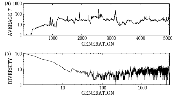
FIG. 2. A stochastic branching process with mutation and selection described in the text approaches a critical state by natural selection. Average total population is \tilde{m}=100 . Simulation started with 100 unique strains whose fitness is drawn from a fitness distribution with T=1 , \sigma=3/2 , and \epsilon_{\max}=1 . The i th strain produces mutants (mutation rate \eta=0.01 ) whose fitness is drawn from a fitness distribution with T_i given by Eq. (19) ( \gamma=2 ). (a) Average temperature of the system stays near the transition point T_c=33 . In early stages, the average temperature increases, indicating initial adaptive evolution. (b) Number of existing strains at each steps (diversity) decreases during initial adaptive evolution. However, further dominance by a few species is suppressed as the system approaches near criticality.
