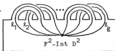
Orientable
