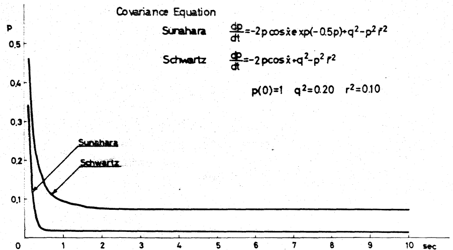
Fig. 5. Error covariance
