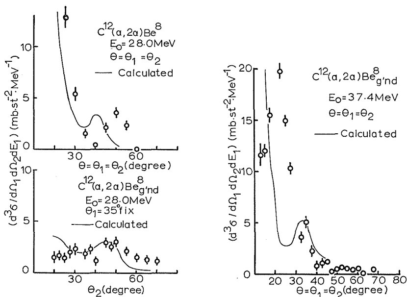
Fig. 38. The calculated angular correlation distributions for the C^{12}(\alpha, 2\alpha)Be^8_{g'nd} ( Q \approx -7.5 MeV) reaction. The experimental angular correlation distributions in this figure are those obtained by the symmetric method ( \theta_1 = \theta_2 ) and when E_1 \approx E_2 at both energies that obtained by the non-symmetric method ( \theta_1 = 35^\circ ) when E_1 \approx E_2 at 28.0 MeV. For calculations and discussions see in text.
