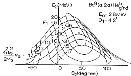
Fig. 6. A kinematical relation of |k_R| vs. ( E_1, \theta_1, E_2, \theta_2 ) for the \text{Be}^9 (\alpha, 2\alpha) \text{He}^5_{g'nd} ( Q \simeq -2.5 MeV) reaction at 28.0 MeV in a non-symmetric geometry ( \theta_1 is fixed at 42^\circ and \theta_2 is varied.)
