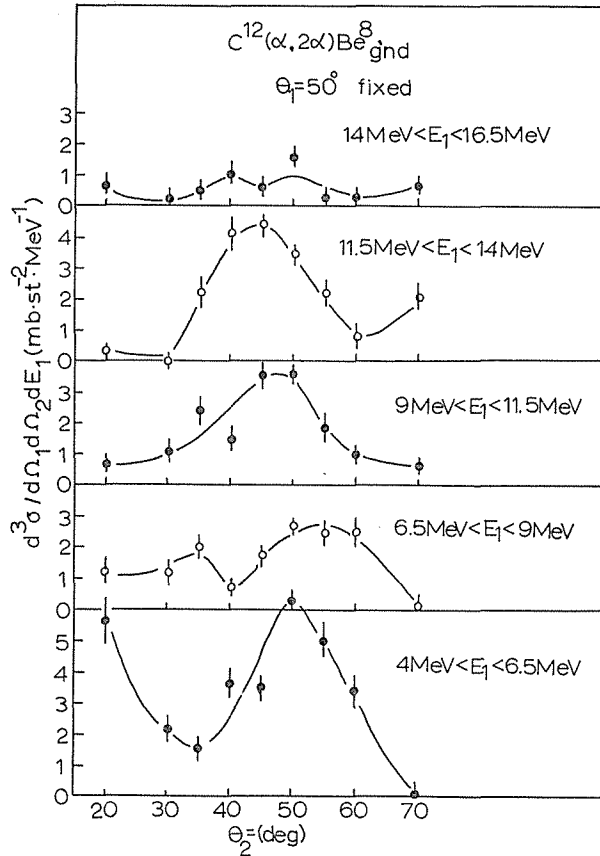
Fig. 28. The angular correlation distributions for the C^{12}(\alpha, 2\alpha)Be^8_{gnd} ( Q \simeq -7.5 MeV) reaction at 28.0 MeV obtained by the non-symmetric method when \theta_1 is fixed at 50^\circ . The distribution is shown for each 2.5 MeV interval of E_1 .
