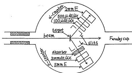
Fig. 7. A schematic diagram of the experimental arrangement for the measurement of the \text{Be}^9(p, p\alpha)\text{He}^5 reaction.
