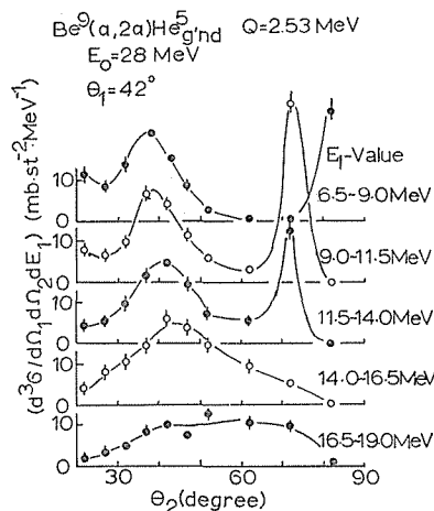
Fig. 12. The angular correlation distributions for the \text{Be}^9(\alpha, 2\alpha)\text{He}^5_{\text{gnd}} ( Q \simeq -2.5 MeV) reaction at 28.0 MeV obtained by the non-symmetric method when \theta_1 is fixed at 42^\circ . The distribution is shown for each 2.5 MeV interval of E_1 .
