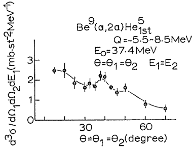
Fig. 18. The angular correlation distributions for the \text{Be}^9(\alpha, 2\alpha)\text{He}^5_{1\text{st}} ( Q \simeq -7.0 MeV) reaction at 37.4 MeV obtained by the symmetric method ( \theta = \theta_1 = \theta_2 ). Only the symmetric energy distribution ( E_1 \simeq E_2 ) is shown.
