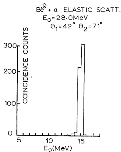
Fig. 4. A single energy spectrum of the elastically scattered alpha-particle from the \text{Be}^9 nucleus when the coincidence measurement was performed.
