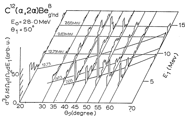
Fig. 44. The E_1 - \theta_2 correlation distribution for the C^{12} ( \alpha , 2 \alpha ) Be^8_{gnd} ( Q \simeq -7.5 MeV) reaction at 28.0 MeV when \theta_1 is fixed at 50^\circ . The solid lines show the energies of the alpha-particles corresponding to the sequential decay process.
