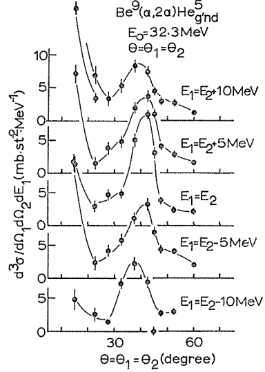
Fig. 15. The angular correlation distributions for the \text{Be}^9(\alpha, 2\alpha)\text{He}^5 ( Q \simeq -2.5 MeV) reaction at 32.3 MeV obtained by the symmetric method ( \theta = \theta_1 = \theta_2 ). The distribution is shown for each 5.0 MeV interval of E_1 .
