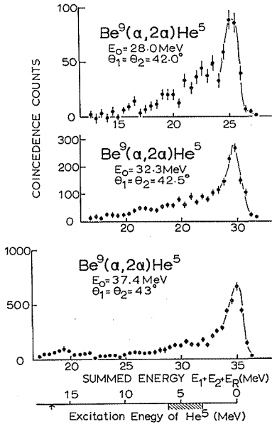
Fig. 10. The summed-energy spectra of the emitted alpha-particles from the \text{Be}^9(\alpha, 2\alpha)\text{He}^5 reactions at 28.0, 32.3 and 37.4 MeV respectively, when both counters are set at the recoilless angles for the Q -value of -2.5 MeV in the symmetric method. The abscissa shows the summed energy ( E_1 + E_2 + E_R ) and the excitation energy of the residual \text{He}^5 nucleus.
