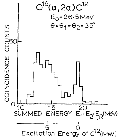
Fig. 32. A summed-energy spectrum of the emitted alpha-particles from the O^{16}(\alpha, 2\alpha)C^{12} reaction at 26.5 MeV, when both counters are set at 35^\circ ( =\theta_1 = \theta_2 ).
