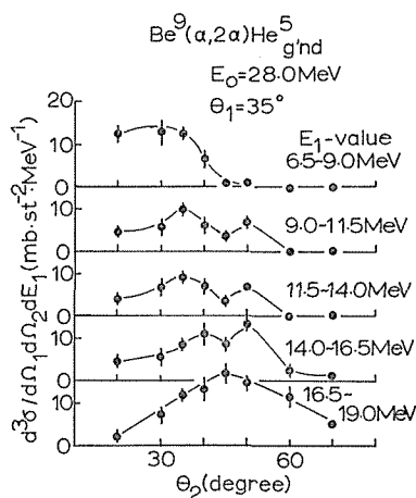
Fig. 13. The angular correlation distributions for the \text{Be}^9(\alpha, 2\alpha)\text{He}^5_{\text{gnd}} ( Q \simeq -2.5 MeV) reaction at 28.0 MeV obtained by the non-symmetric method when \theta_1 is fixed at 35^\circ . The distribution is shown for each 2.5 MeV interval of E_1 .
