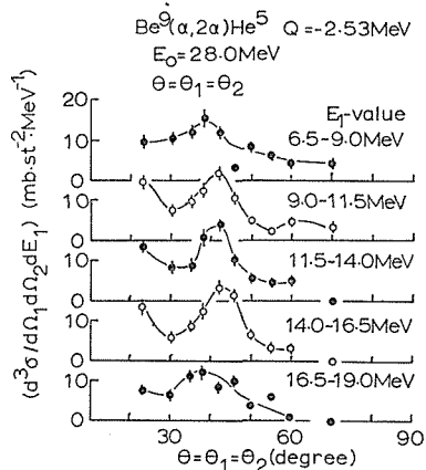
Fig. 11. The angular correlation distributions for the \text{Be}^9(\alpha, 2\alpha)\text{He}^5_{g,nd} ( Q \simeq -2.5 MeV) reaction at 28.0 MeV obtained by the symmetric method ( \theta_1 = \theta_2 ). The distribution is shown for each 2.5 MeV interval of E_1 .
