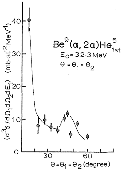
Fig. 16. The angular correlation distributions for the \text{Be}^9(\alpha, 2\alpha)\text{He}^5_{1\text{st}} ( Q \simeq -7.0 MeV) reaction at 32.3 MeV obtained by the symmetric method ( \theta = \theta_1 = \theta_2 ). Only the symmetric energy distribution ( E_1 \simeq E_2 ) is shown.
