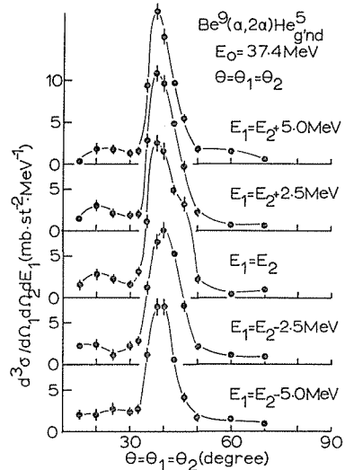
Fig. 17. The angular correlation distributions for the \text{Be}^9(\alpha, 2\alpha)\text{He}^5_{\text{gnd}} ( Q \simeq -2.5 MeV) reaction at 37.4 MeV obtained by the symmetric method ( \theta = \theta_1 = \theta_2 ). The distributions is shown for each 2.5 MeV interval of E_1 .
