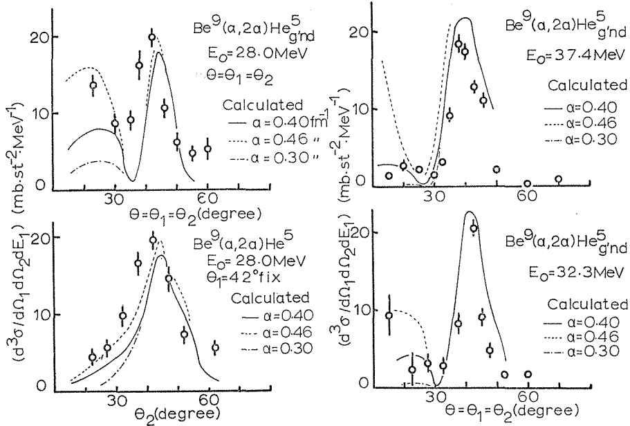
Fig. 36. The calculated angular correlation distributions together with the experimental values for the \text{Be}^9(\alpha, 2\alpha)\text{He}^5_{\text{gnd}} reaction. The experimental angular correlation distribution in this figure are that obtained by the symmetric method ( \theta_1=\theta_2 ) and when E_1 \simeq E_2 at each energy and that obtained by the non-symmetric method ( \theta_1=42^\circ ) and when E_1 \simeq E_2 at 28.0 MeV. For calculations and discussions see in text.
