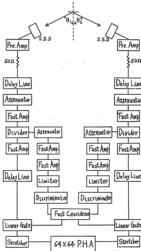
Fig. 2. A block diagram of the electronic system for the measurement of the (\alpha, 2\alpha) reactions.
