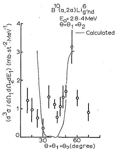
Fig. 37. The calculated angular correlation distribution together with the experimental values for the B^{10} (\alpha, 2\alpha) Li^6_{g.nd} ( Q \simeq -4.5 \text{ MeV} ) reaction. The experimental angular correlation distribution in this figure is that obtained by the symmetric method ( \theta_1 = \theta_2 ) and when E_1 \simeq E_2 at 28.4 \text{ MeV} . For calculations and discussions see in text.
