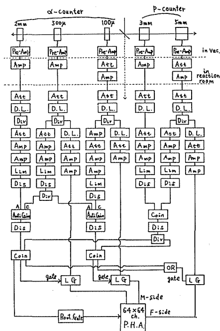
Fig. 8. A block diagram of the electronic system for the measurement of the \text{Be}^9(p, p\alpha)\text{He}^5 reaction.
