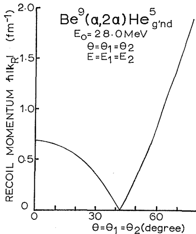
Fig. 5. A kinematical relation of |k_R| vs. ( E_1, \theta_1, E_2, \theta_2 ) for the \text{Be}^9 (\alpha, 2\alpha) \text{He}^5_{g'nd} ( Q \simeq -2.5 MeV) reaction at 28.0 MeV in the symmetric geometry ( \theta = \theta_1 = \theta_2 , k = |k_1| = |k_2| ).
