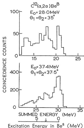
Fig. 24. The summed-energy spectra of the emitted alpha-particles from the C^{12}(\alpha, 2\alpha)Be^8 reaction at 28.0 and 37.4 MeV respectively, when both counters are set at the recoilless angles for the Q -value of -7.5 MeV in the symmetric method. The abscissa shows the summed energy ( E_1 + E_2 + E_R ) and the excitation energy of the residual Be^8 nucleus.
