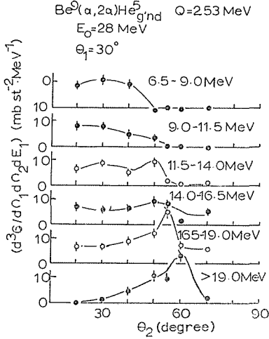
Fig. 14. The angular correlation distributions for the \text{Be}^9(\alpha, 2\alpha)\text{He}^5_{\text{gnd}} ( Q \simeq -2.5 MeV) reaction at 28.0 MeV obtained by the non-symmetric method when \theta_1 is fixed at 30^\circ . The distribution is shown for each 2.5 MeV interval of E_1 .
