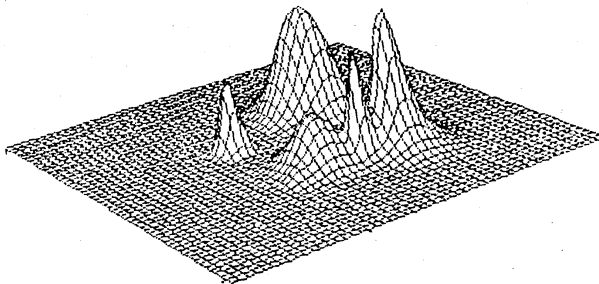
(g) \theta_{\text{net}} = 19.00, \theta_{\text{total}} = 21.74, \rho = 0.874
