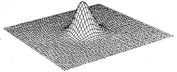
(d) \theta_{\text{net}} = 6.231, \theta_{\text{total}} = 6.231, \rho = 1.000
