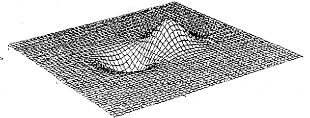
(f) \theta_{\text{net}} = -8.2 \times 10^{-7}, \theta_{\text{total}} = 6.613, \rho = -1.3 \times 10^{-7}
