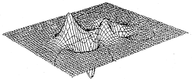
(h) \theta_{\text{net}} = -2.93, \theta_{\text{total}} = 12.60, \rho = -0.233
