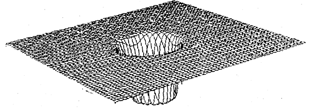
(b) \theta_{\text{net}} = -6.610, \theta_{\text{total}} = 6.613, \rho = 0.999
