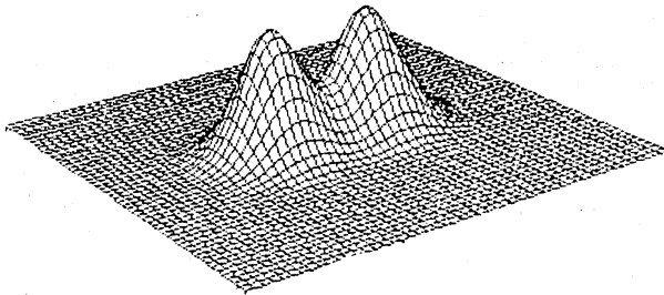
(e) \theta_{\text{net}} = 6.610, \theta_{\text{total}} = 6.613, \rho = 0.999
