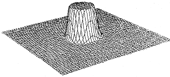
(a) \theta_{\text{net}} = 6.610, \theta_{\text{total}} = 6.613, \rho = 0.999
