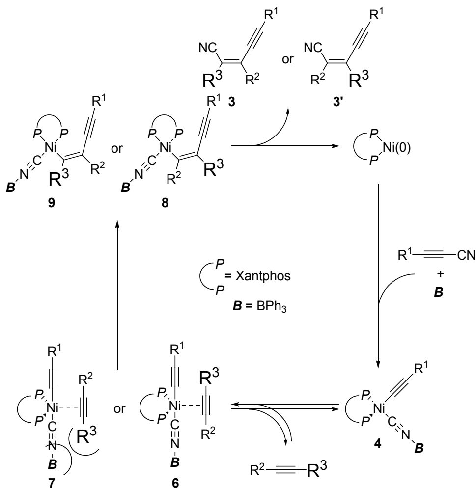
Scheme 3. Plausible mechanism for the nickel/ \text{BPh}_3 -catalyzed alkynylcyanation of alkynes.
