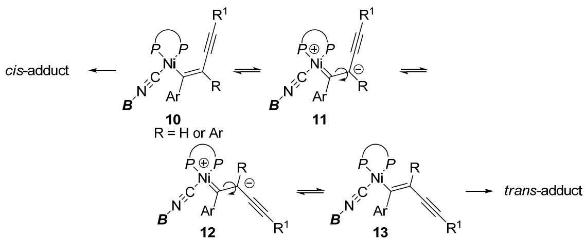
Scheme 4. Plausible mechanism for the formation of trans -alkynylcyanation products ( 3aj–3al ).
