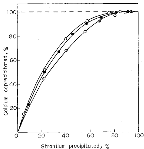
Fig. 2. The effect of acetate ion. Sr: 0.025M, Ca: 10^{-6} M, pH: 4.00 acetate: \circ —; 0.5M, \lambda=2.97 , \bullet —; 1.0M, \lambda=2.71 , \odot —; 2.0M, \lambda=2.22
