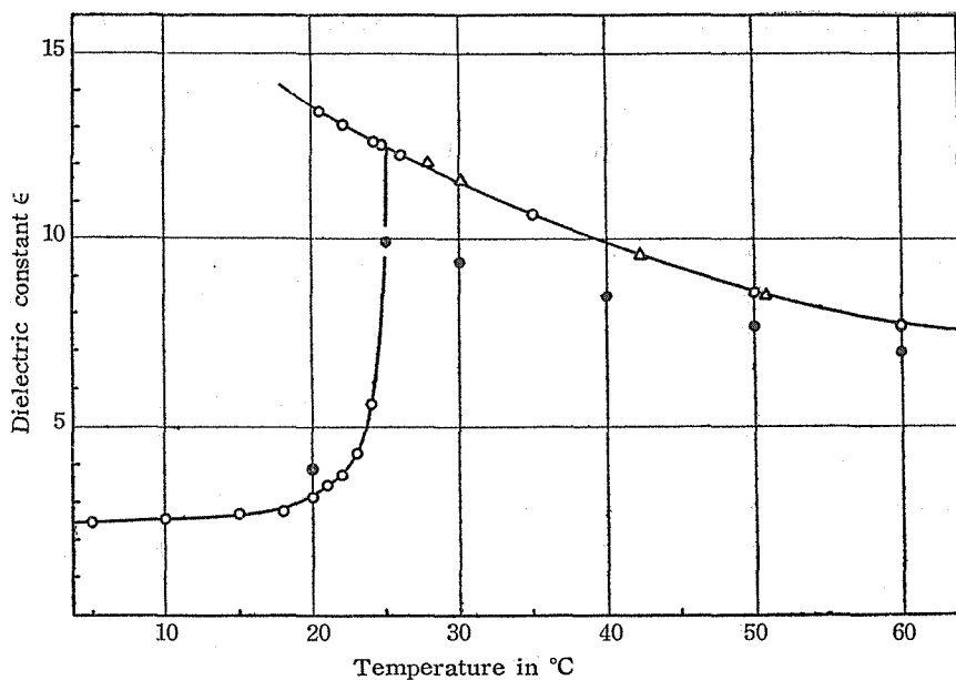
Fig. 2. Dielectric constant of t -butanol versus temperature. (○ This work, \triangle Harris et al. 14) , ● Åkerlöf 9) )
