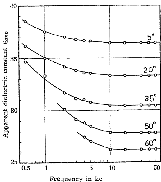
Fig. 3. The variation of apparent dielectric constant \epsilon_{app} of methanol with frequency.
