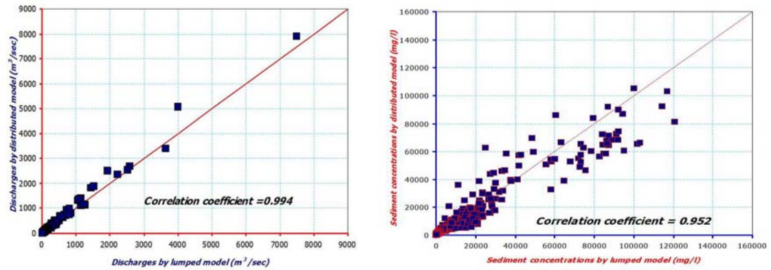
Fig. 12 Comparison of simulated outflow discharges and sediment concentrations by lumped model and distributed model. The solid line is 1 to 1.
