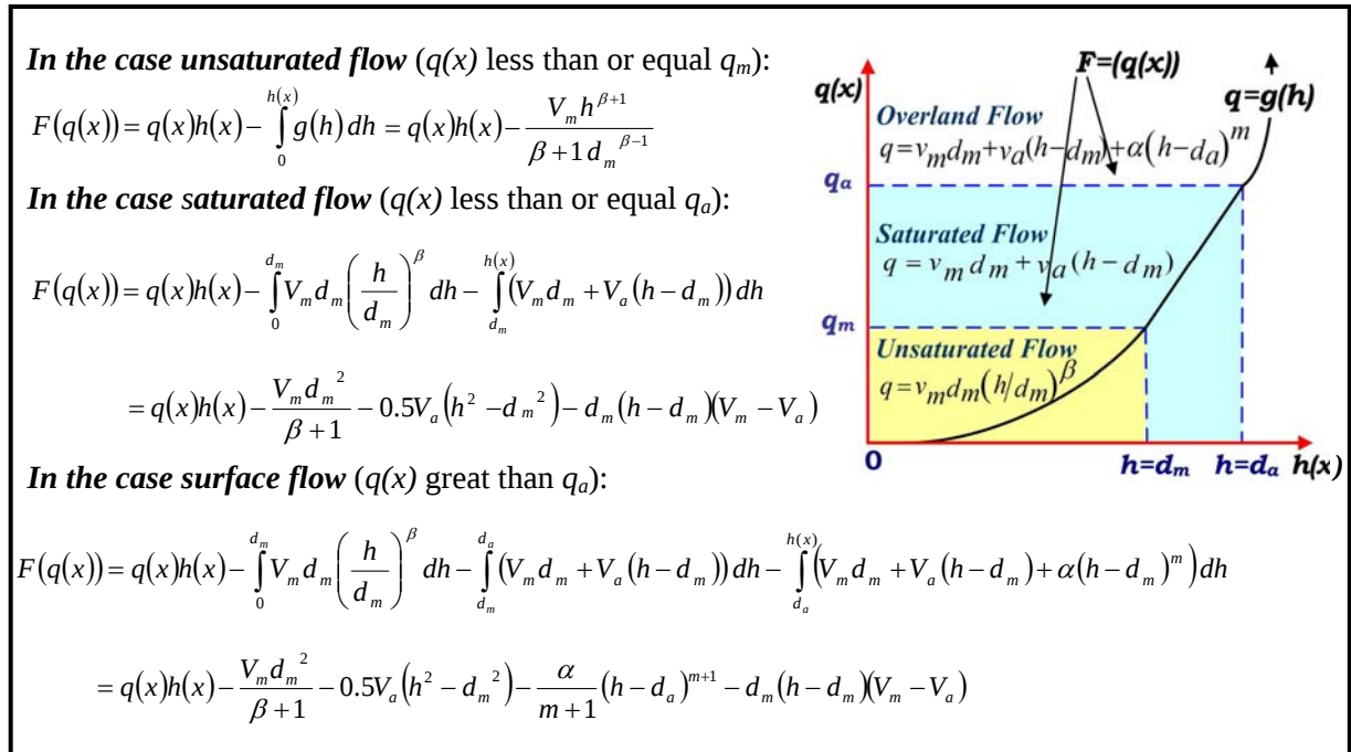
Fig. 7 Schematic drawing of q , h , and F relationship.
