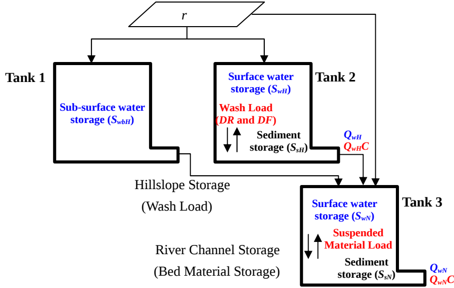
Fig. 6 Schematic diagram of the lumped sediment runoff model at catchment scale.
