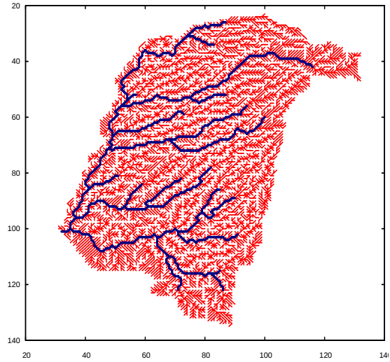
Fig. 9 Flow direction image with river channel network in Lesti River catchment.
