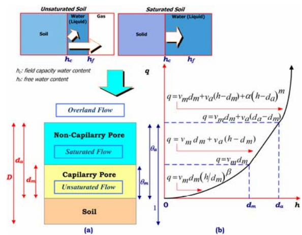
Fig. 2 (a) Concept of hillslope soil layer structure and (b) stage-discharge relationship of CDRMV3.
