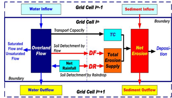
Fig. 3 Schematic diagram of the physically based sediment runoff model at a grid-cell scale.
