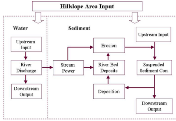
Fig. 4 River channel erosion and deposition mechanism for fine sediment particle.
