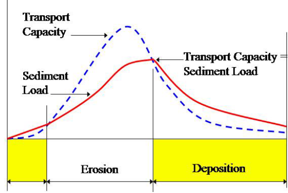
Fig. 5 Relation of deposition to transport capacity and sediment production on hillslopes or river channels.
