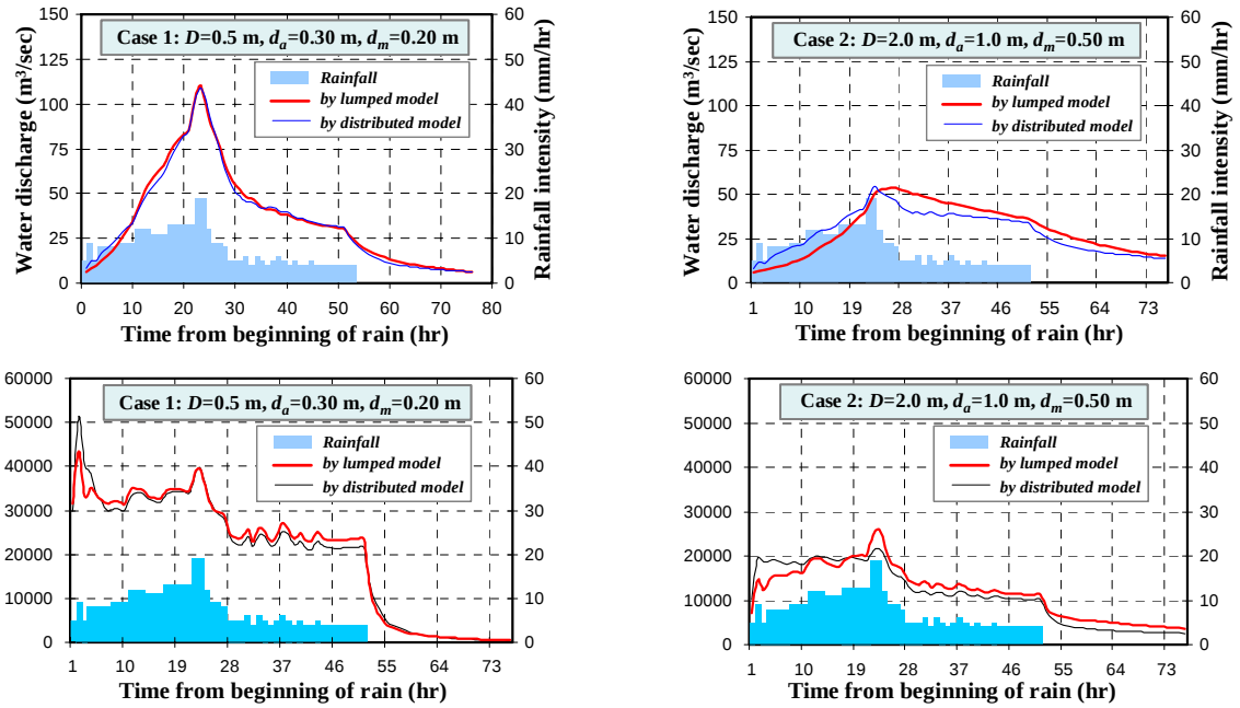
Fig. 11 Computed water discharges and sediment concentrations with different combinations soil thickness ( D ) by using original distributed sediment runoff model and it lumped model version.
