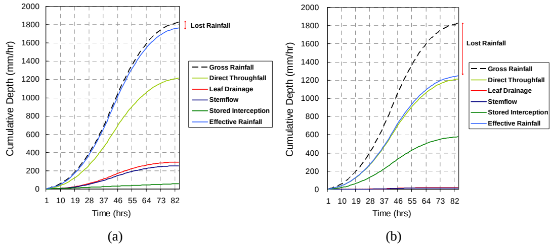
Fig. 10 Simulation the division of cumulative gross rainfall into leaf drip, direct throughfall, stem flow, and effective rainfall under; (a) low interception storage, and (b) high interception storage.
