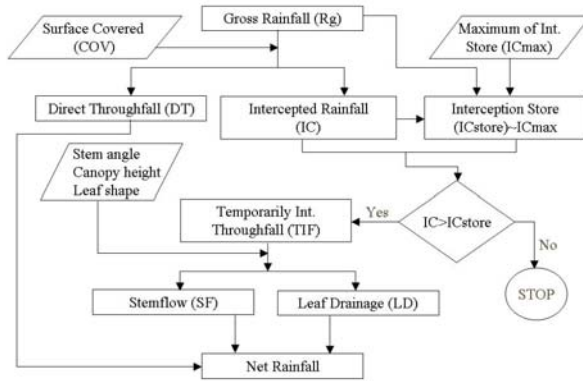
Fig. 1 Schematic diagram of rainfall interception process.
