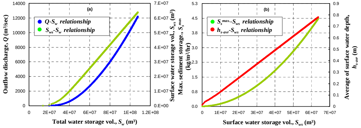
Fig. 8 (a) Plots of discrete relationships between Q-S_w and S_{ws}-S_w ; and (b) discrete relationships between S_s^{max}-S_{ws} and h_{s-avr}-S_{ws} .
