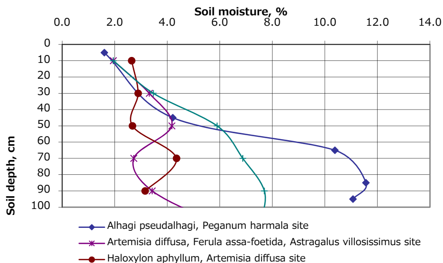
Figure 4. Dynamics of soil moisture under different desert plant communities.
