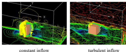
Fig. 18 Analysis of wind fields around bluff body with artificially generated fluctuational wind for boundary conditions
