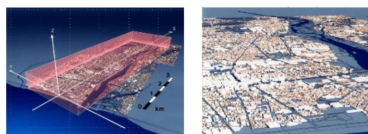
Fig. 11 Configuration of surface roughness around Hiratsuka city for the wind field simulation with canopy model
