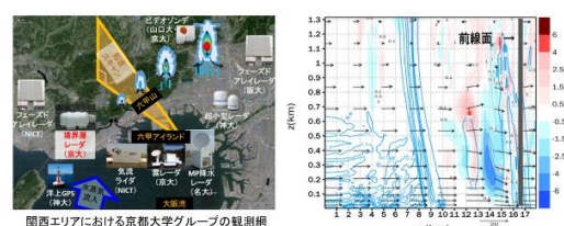
Fig. 8 Observation of wind field under cumulus convection and its numerical simulation
