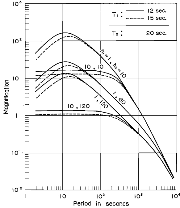
Fig. 5.7. Calculated magnification curve of the Askaniya gravimeter No. 111 as a seismometer.
