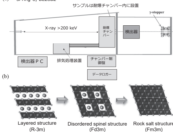
Fig. 1. (a) Overall view of the operando CT measurement system and (b) Phase transition of \text{LiMO}_2 cathode from layered structure to spinel structure, rock salt structure.
