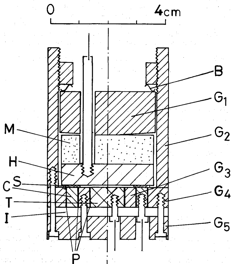
Fig. 1. Design of the dielectric cell for deformable solids.
