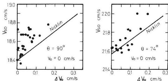
Fig. 7.19 Correlative representation of water flow caused by bubble expansion
