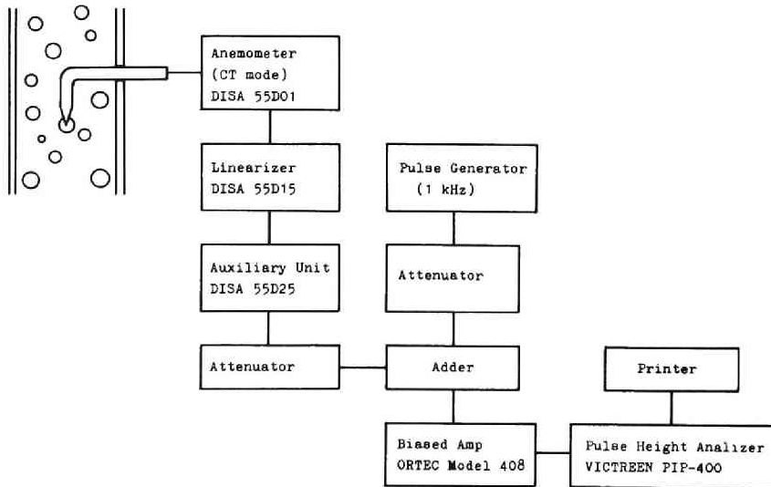
Fig. 2.7 Schematic of anemometer method
