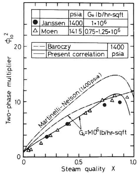
Fig. 6.10 Correlative representation of experimental pressure drop data for steam-water
