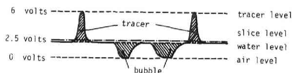
Fig. 2.9(a) Probe signal and slice level in tracer technique
