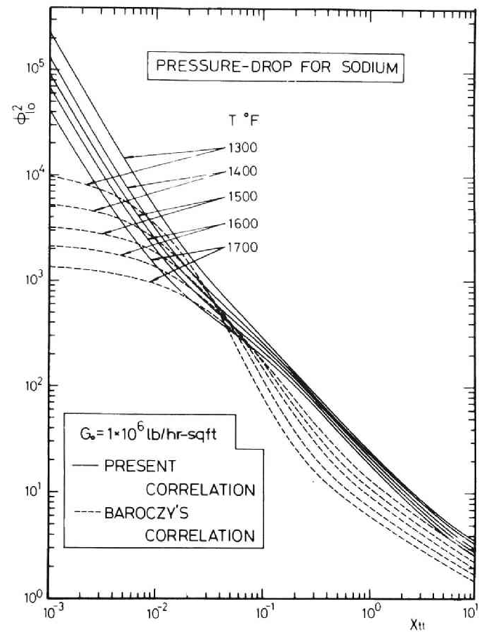
Fig. 6.21 Pressure level and temperature effects for sodium at G_0 = 1 \times 10^6 \text{ lb/hr} \cdot \text{ft}^2
