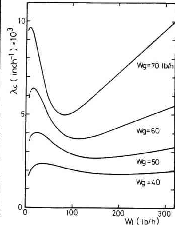
Fig. 8.6 Predicted coefficient calculated from data of Cousins et al.[8]
