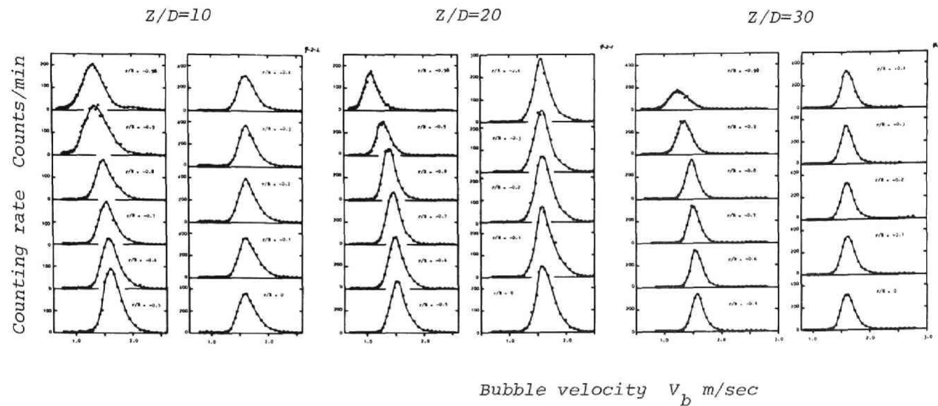
Fig. 4.42 Axial and radial variations of bubble velocity spectrum ( V_0 = 1.03 m/sec, X = 0.0170 % : bubble flow)
