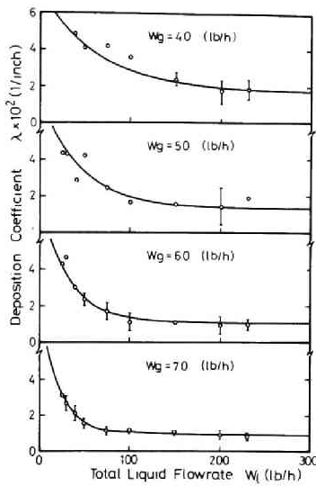
Fig. 8.4 Deposition coefficient calculated from data of Cousins et al.[8]
