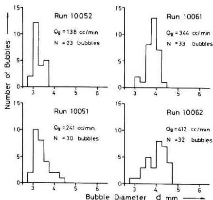
Fig. 3.30 Histogram of equivalent-spherical-diameter of bubbles ( V_O = 0.74 m/sec)
