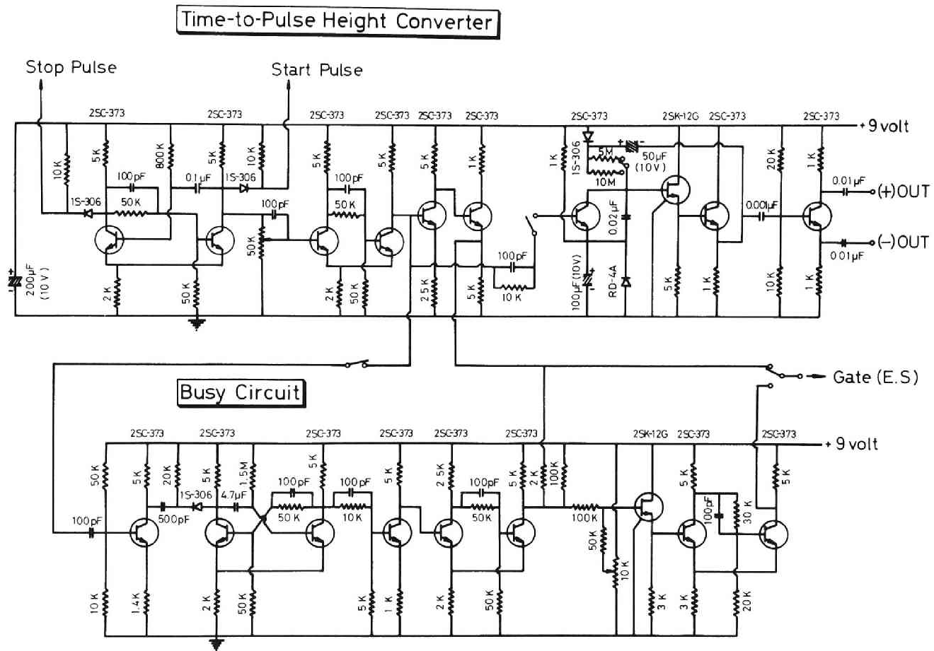
Fig. 2.2(b) Wiring diagram of electronic circuit
