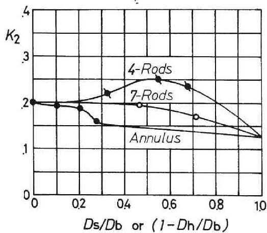
Fig. 7. 13 Flow parameter K_2 for various types of flow channel ( V_0 \geq 0.5 m/sec)
