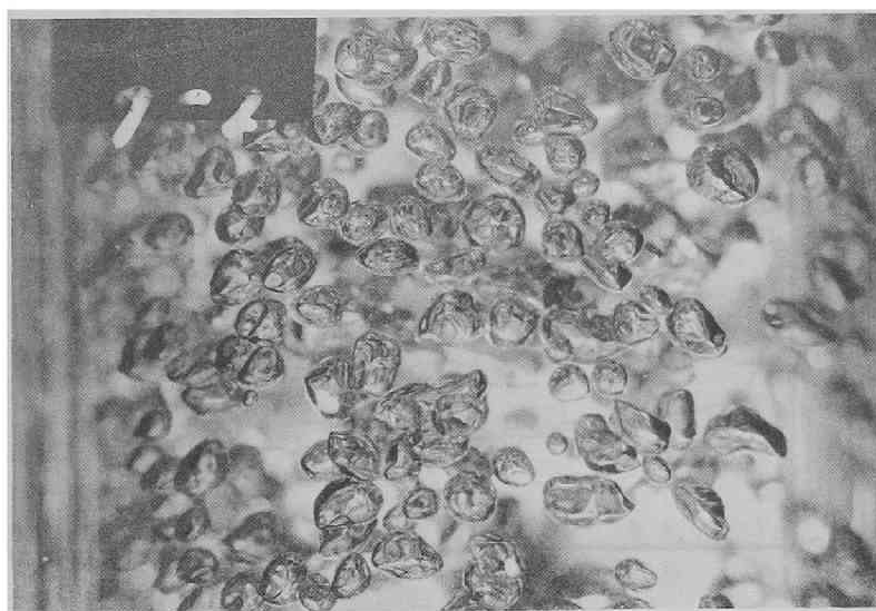
(b) Bubble flow (V_o = 1.03 \text{ m/sec}, X = 0.0170 \%, Z/D = 22.5)
