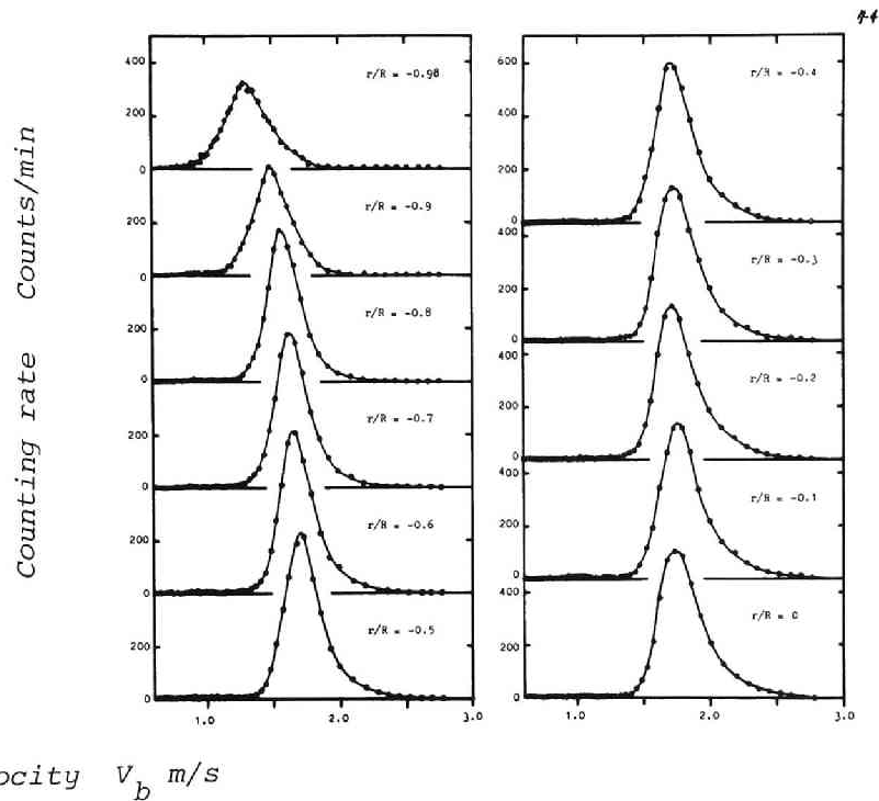
Fig. 4.56 Bubble velocity spectrum (Bubble flow : V_O = 1.03 m/sec, X = 0.0341 %, Z/D = 30 )
