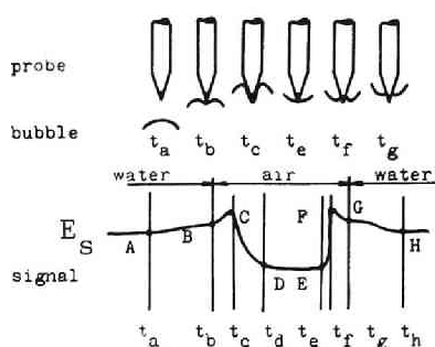
Fig. 2.8(a) Passage of a single air bubble past the conical hot-film probe
