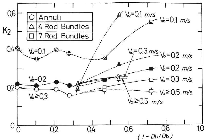
Fig. 7.14 Flow parameter K_2 for various water velocity and types of flow channel ( V_0 < 0.5 m/sec)
