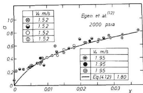
Fig. 4.9 Correlative representation of experimental void fraction for steam-water (bubble flow)
