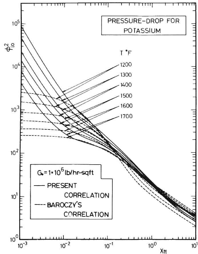
Fig. 6.20 Pressure level and temperature effects for potassium at G_0 = 1 \times 10^6 \text{ lb/hr} \cdot \text{ft}^2
