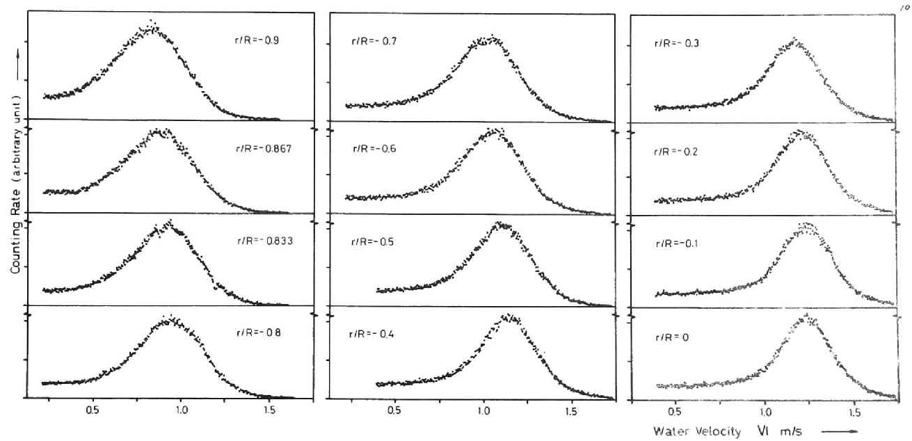
Fig. 4.76 Water velocity spectrum (Transition flow : V_O = 0.74 m/sec, X = 0.0478 %, Z/D = 30 )
