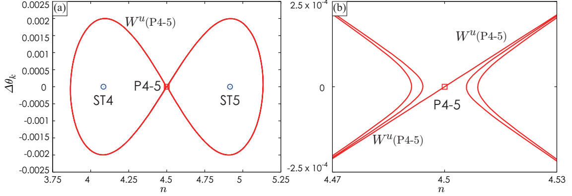
Figure 4.3: Unstable manifolds of P4-5 at \beta_2 = 0.001 , \mathcal{H} = 17 .
