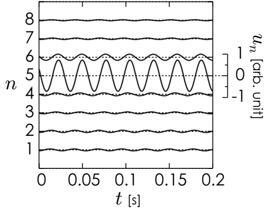
(a) ILM at n = 5
