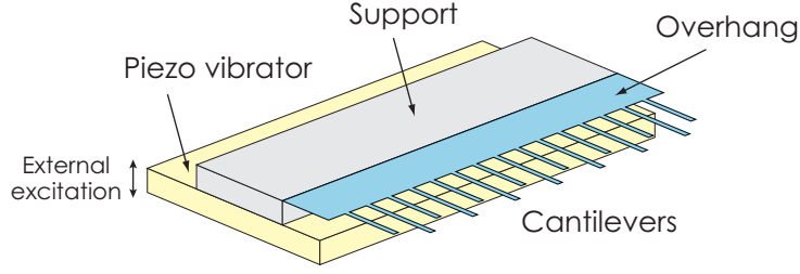
Figure 1.1: Schematic configuration of a micro-cantilever array fabricated by M. Sato et al. [29]. Short and long cantilevers are coupled by the overhang region which is a flexible thin film. To excite the cantilevers, the piezo vibrator is attached to the support.
