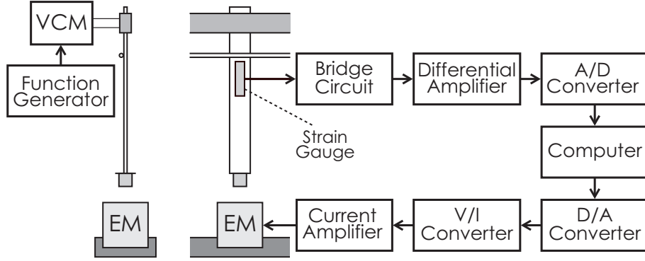
Figure 6.6: Experimental setup.
