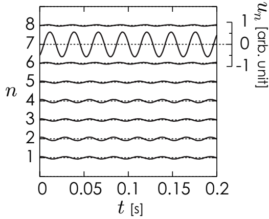
(c) ILM at n = 7
