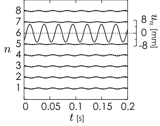
(b) ILM at n = 6
