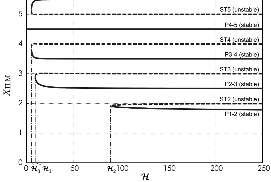
Figure 3.7: Bifurcation diagram for coexisting ILMs at \beta_2 = 0.01 . \mathcal{H}_0 \simeq 5.06 , \mathcal{H}_1 \simeq 9.09 , \mathcal{H}_2 \simeq 88.8 .
