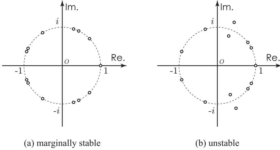
Figure 2.7: Floquet multipliers for (a) marginally stable and (b) unstable ILMs [53].
