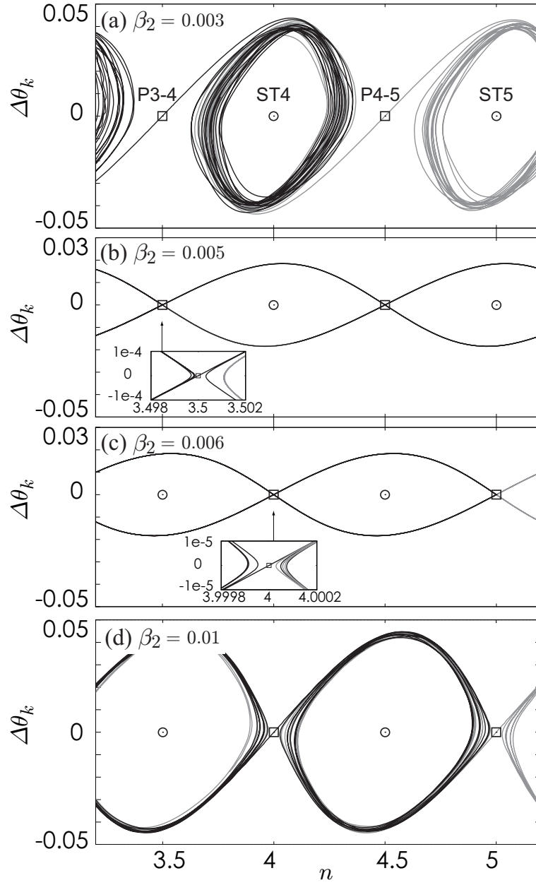
Figure 4.5: Coexisting ILMs and unstable manifolds at \beta_2 = 0.003 (a), 0.005(b), 0.006(c), and 0.01(d). Structure of the vicinity of an unstable ILM is shown in the insets. Unstable manifolds are located very close to the unstable ILM. There is no homo- or heteroclinic connection.
