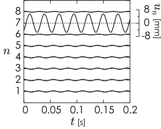
(c) ILM at n = 7
