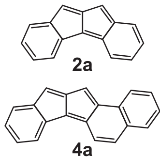
FIG. 2. Molecular structures of 2a and 4a
