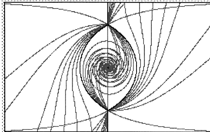
Figure 1: The Stokes lines for various phases of \nu . The bounded Stokes lines from i to -i for \text{ph}(\nu) = \pm \frac{1}{2}\pi are the boundary of the bounded (spiral) and the unbounded (radial) domains.
