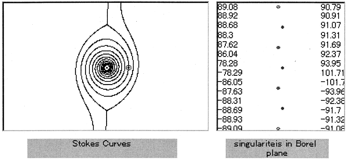
Figure 5: The left shows the point z = 0.5 is on the spiral Stokes line for \theta^{(n,n+3)} = 86.04 \text{ deg} . The right is the image of the saddles on the Borel plane. The figures in the right box are degrees of the angles between the singularities.
