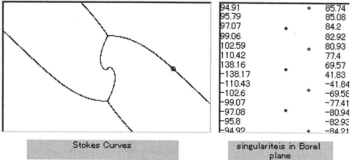
Figure 3: The left shows the point z = 2 is exactly on the radial Stokes line for \theta = 41.84 deg (rounded). The right is the image of the saddles on the Borel plane. The figures in the right box are degrees of the angle between the singularities.
