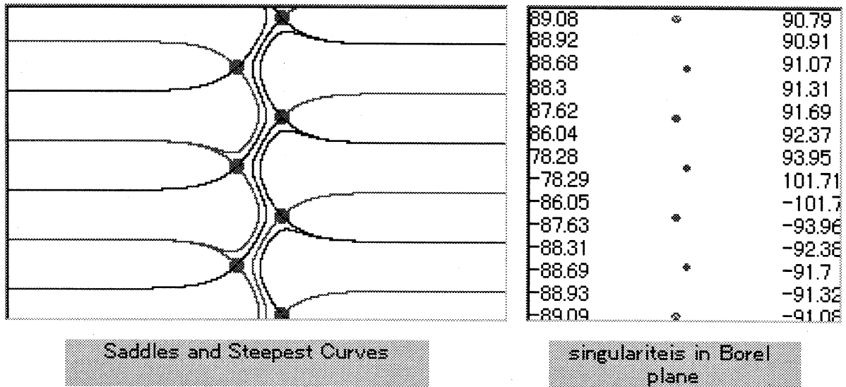
Figure 6: The left is a figure of saddles and steepest curves for \theta^{(n,n+3)} = 86.04 deg (roughly rounded). The steepest descents creep up from the saddles w^{(n)} to hit the adjacent saddles w^{(n+3)} .
