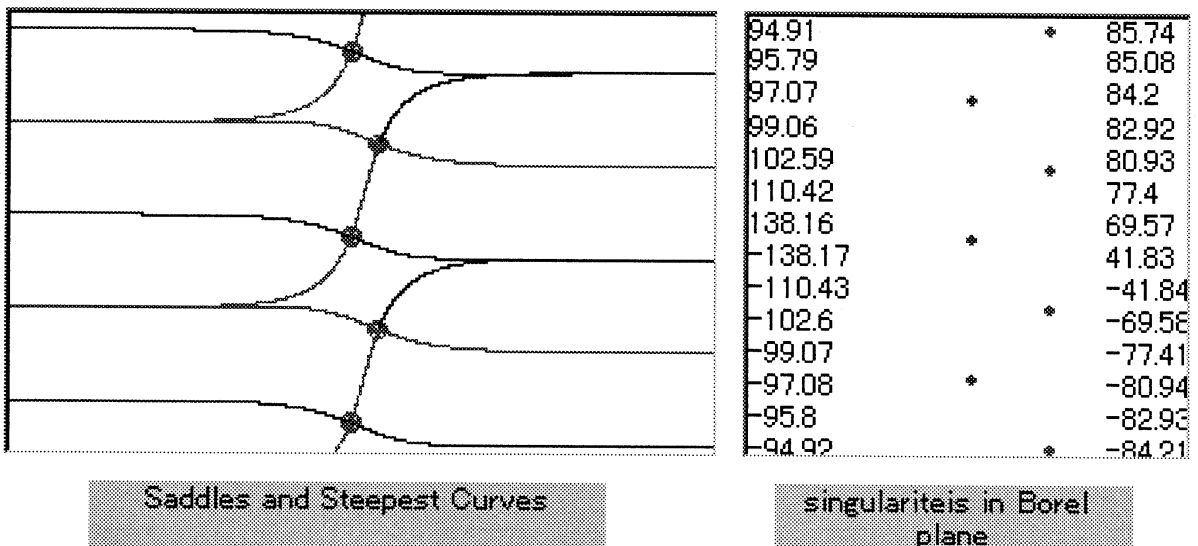
Figure 4: The left is a figure of saddles and steepest curves for \theta^{(n,n-1)} = -41.84 deg (round) when z = 2 . The right is the image of the saddles on the Borel plane. The figures in the right box are degrees of the angle between the singularities.
