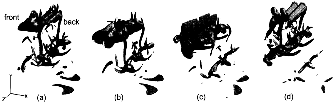
Fig. 7: Isosurfaces of the magnitude of the vorticity ( |\nabla \times \mathbf{u}|c/u_{\max} = 1.5 ) around the 3D flapping wings at \phi = 0^\circ ; (a) t = 5.25T , (b) t = 5.50T , (c) t = 5.75T , and (d) t = 6.00T .
