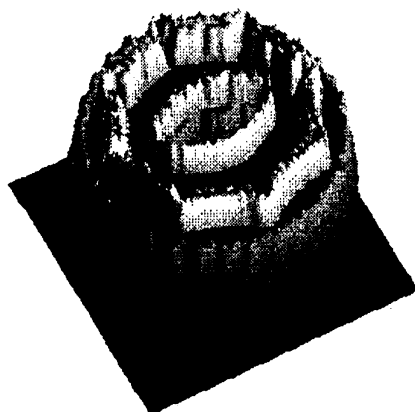
Figure 5: The graph of z \mapsto \frac{\partial T}{\partial p}(h_1, h_2, 1/2, z) . A complex analogue of the Takagi function.
