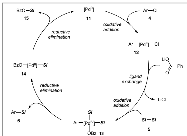
Figure 1 Proposed Reaction Mechanism
