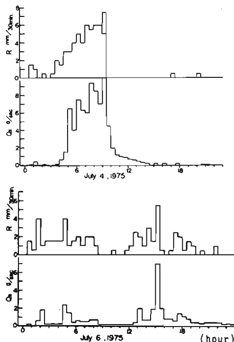
Fig. 20. Rainfall and sediment discharge at Hirudani Branch Station.
