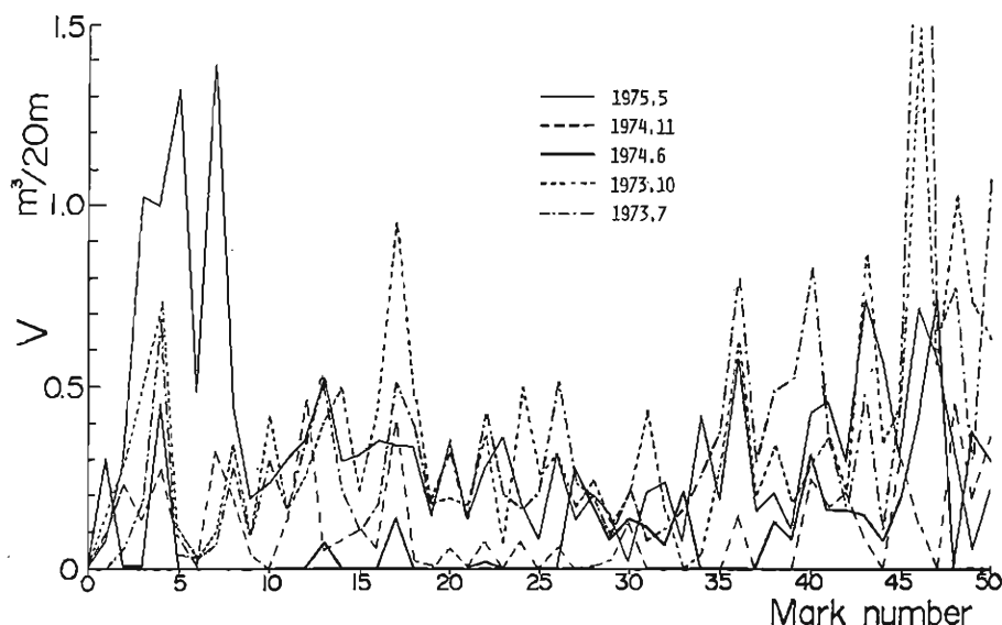
Fig. 25. Sediment storage variation for every 20 m on the course of the Hirudani stream channel.
