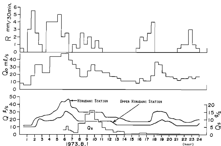
Fig. 14. 1973.8. Flood. Q_o : Spring discharge.
