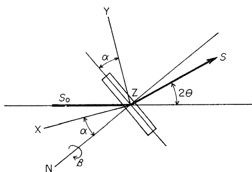
Fig. 1. Geometry for transmission technique.
