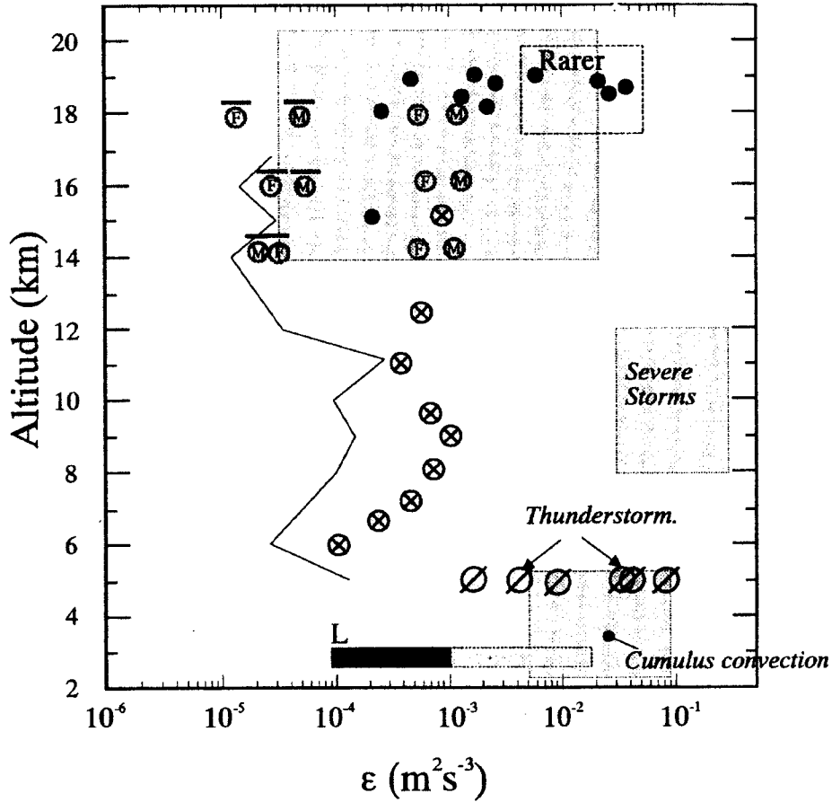
Figure 1.1: Various in-situ measurements of kinetic energy dissipation rates in the troposphere [Hocking and Mu, 1997]. \otimes , \bullet , and \oslash show the results of Kung [1966], Vinnichienko and Dutton [1969] and Bohne [1981], respectively. The line shows the results of Crane [1980]. The shaded areas represent the results of Chen [1974]. \oplus and \odot are the values of \epsilon reported by Lilly et al. [1974] over flatland/water and mountainous areas, respectively. The data of Lilly et al. [1974] with and without the overline indicate, respectively, the average over the whole atmosphere and in only the turbulent layer. The rectangle indicated by 'L' shows the results of Lee et al. [1988]. About 90% of their data lay in the black rectangular region.
