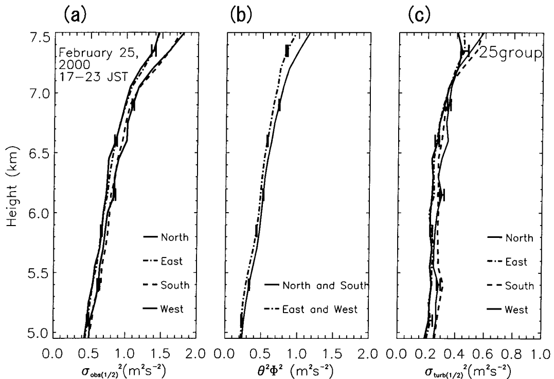
Figure 3.5: As in Figure 3.1, but for 17–23 LT on February 25, 2000.
