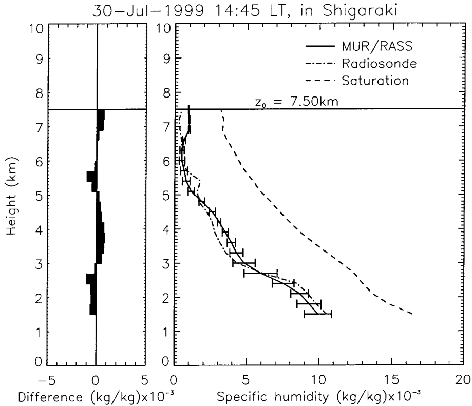
Figure 6.5: Comparison of q (right) from MU radar–RASS observations (solid) and a radiosonde (dash dot) launched at 14:36 LT on July 30, 1999. The error bars show the s.d. for the radar results. Note that the dashed line indicates the saturation line. The left panel shows the difference in q between the radar and radiosonde results.
