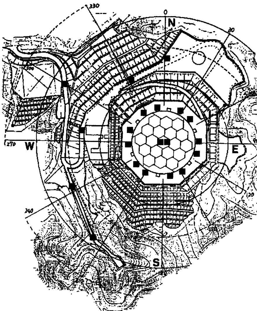
Figure 2.8: The positions of electro-dynamic loudspeakers with the hyperbolic horn. The location of each acoustic source is indicated by the black box.
