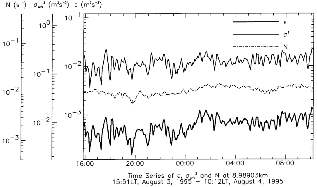
Figure 4.10: Profiles of \epsilon with the spectral with (thick solid), \sigma_{turb}^2 (solid), and N (short-dashed) between 16:00 LT on August 3 and 10:00 LT on August 4. The vertical axis is scaled logarithmically and its extent is 10^3 .
