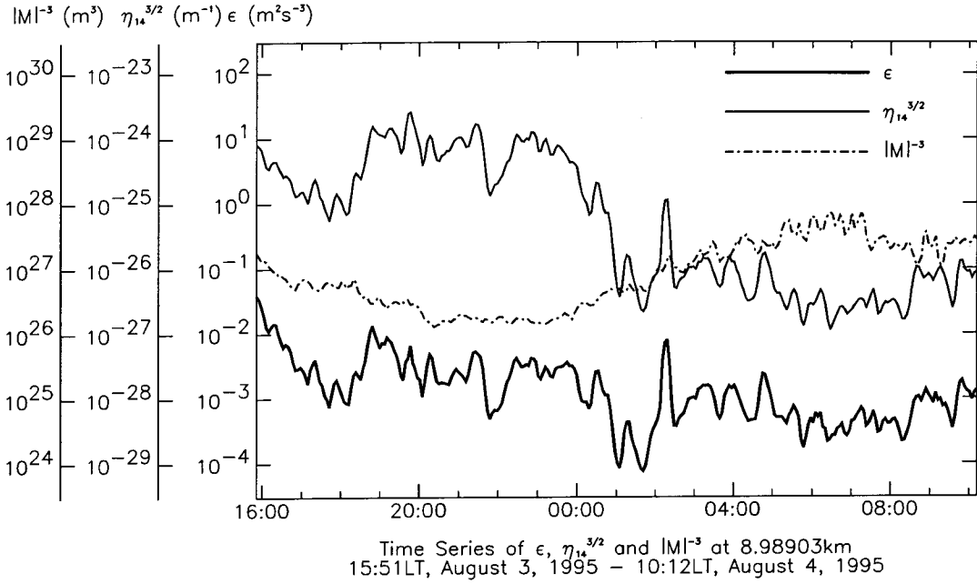
Figure 4.11: The same as Figure 4.10 except profiles of \epsilon are with the echo power (thick solid), \bar{\eta}_{14}^{3/2} (solid), and M^{-3} (short-dashed). The extent of the vertical scale is 10^7 .
