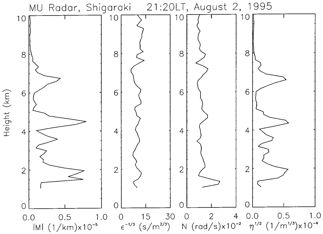
Figure 5.1: Profiles of |M| , \epsilon^{-1/3} , N and \sqrt{\eta_{turb}} (from left to right) calculated from the MU radar-RASS observations at 21:20 on August 2, 1995.
