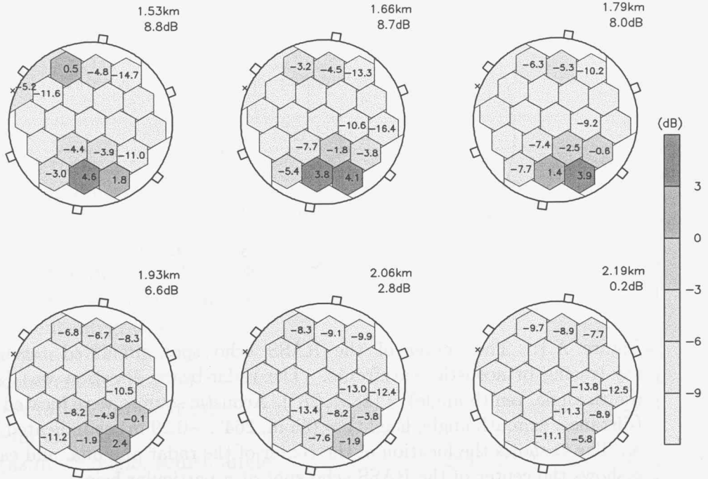
Figure A.3: Distribution of RASS echo intensity ( S/N ) observed by each sub-array at 23:07 LT on December 18, 1995. The radar beam direction was (azimuth angle, zenith angle) = (270°, 28°). The altitude and total S/N are shown at the upper right of the MU radar antenna. S/N was corrected by being multiplied by a factor of r^{-2} . The \times shows the location of the acoustic sources.
