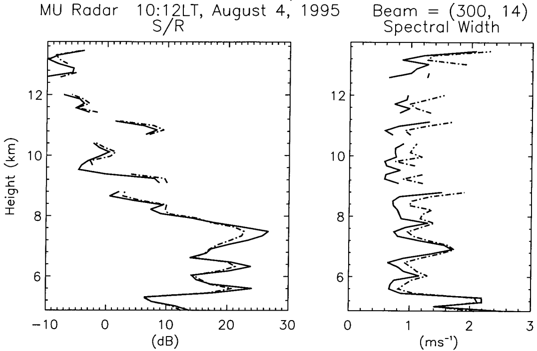
Figure 4.3: Profiles of S/N (left) and spectral width (right) at 10:12 LT on August 4, estimated by Gaussian and the moment methods shown by the solid and short-dashed lines, respectively.
