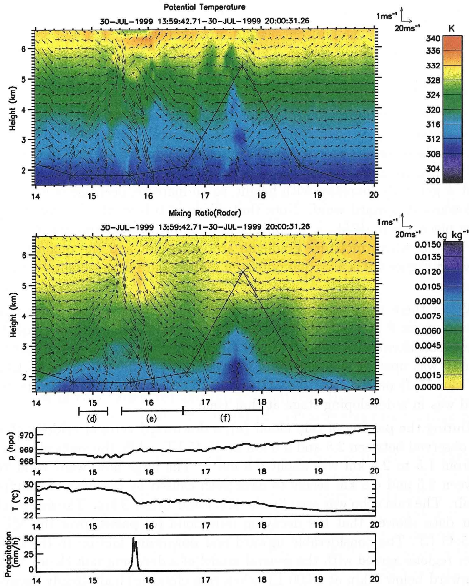
Figure 6.9: Time-height distribution of \theta (top) and q_R (middle) observed by the MU radar-RASS from 14:00 to 20:00 LT on July 30, together with the horizontal and vertical wind velocities indicated by vectors. The cloud-top height obtained by GMS is indicated by asterisks connected by the line. The three panels at the bottom show the time variation of the surface pressure, temperature and precipitation observed at the MU radar. (d), (e) and (f) show the timing of rain clouds passing.
