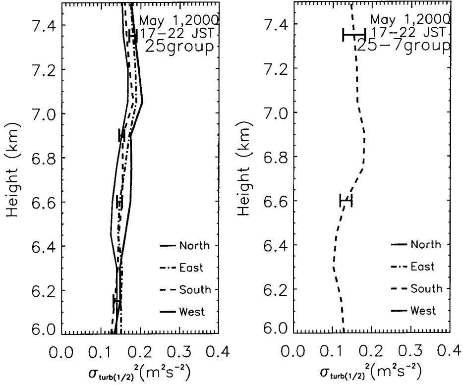
Figure 3.4: \sigma_{\text{turb}}^2 profiles for 17–22 LT on May 1, 2000, for the 1BW method with the 25-group (left), and 2BW method with the 25- and 7-group pair (right). The profile for only the south azimuth is shown.
