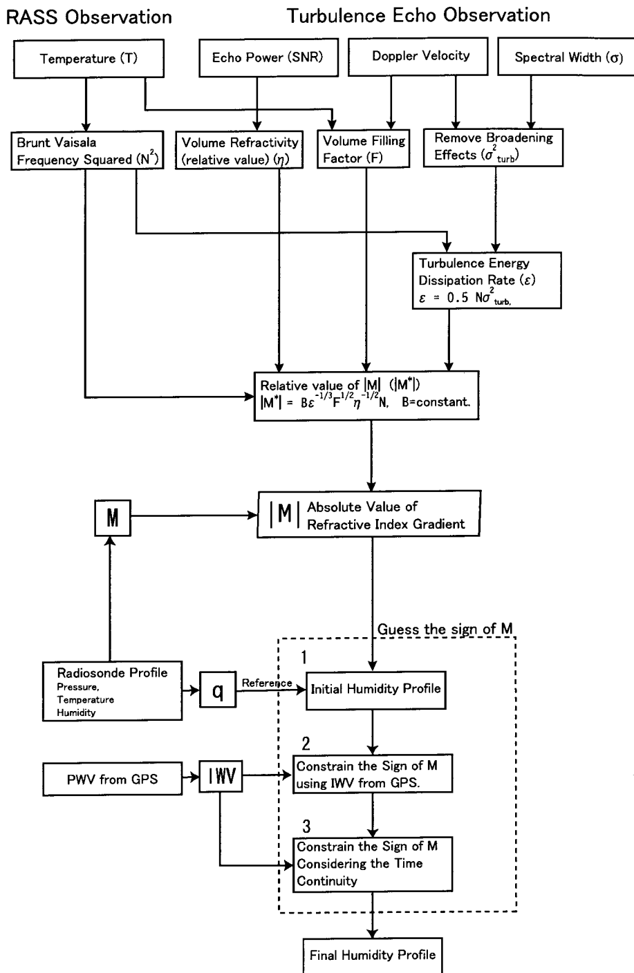
Figure 6.1: Block diagram of an improved retrieval method for estimating q profiles.
