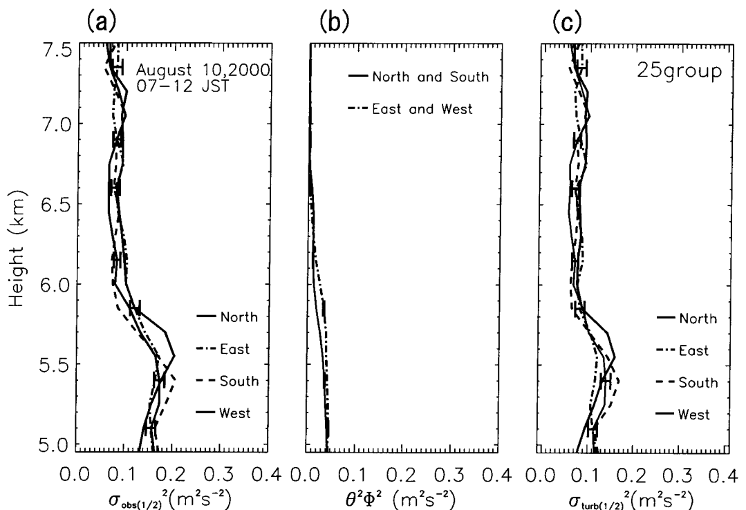
Figure 3.1: Data profiles for 7-12 LT on August 10, 2000, for the 1BW method, with the 25-subarrays group. (a) Observed spectral widths \sigma_{obs}^2 in the cardinal azimuths. (b) \sigma_{corr}^2 for the meridional (North and South) and zonal (East and West) beams. (c) \sigma_{turb}^2 = \sigma_{obs}^2 - \sigma_{corr}^2 for the cardinal azimuths.
