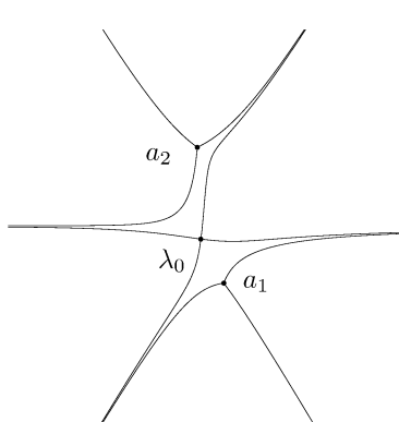
Figure 13. Stokes curves of (SL_{II}) at t = t_1 when c = i .
