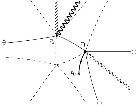
Figure 8. Integration path from \tau_1 to t (near t_0 ).
