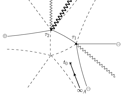
Figure 9. Integration path from \infty to t (near t_0 ).
