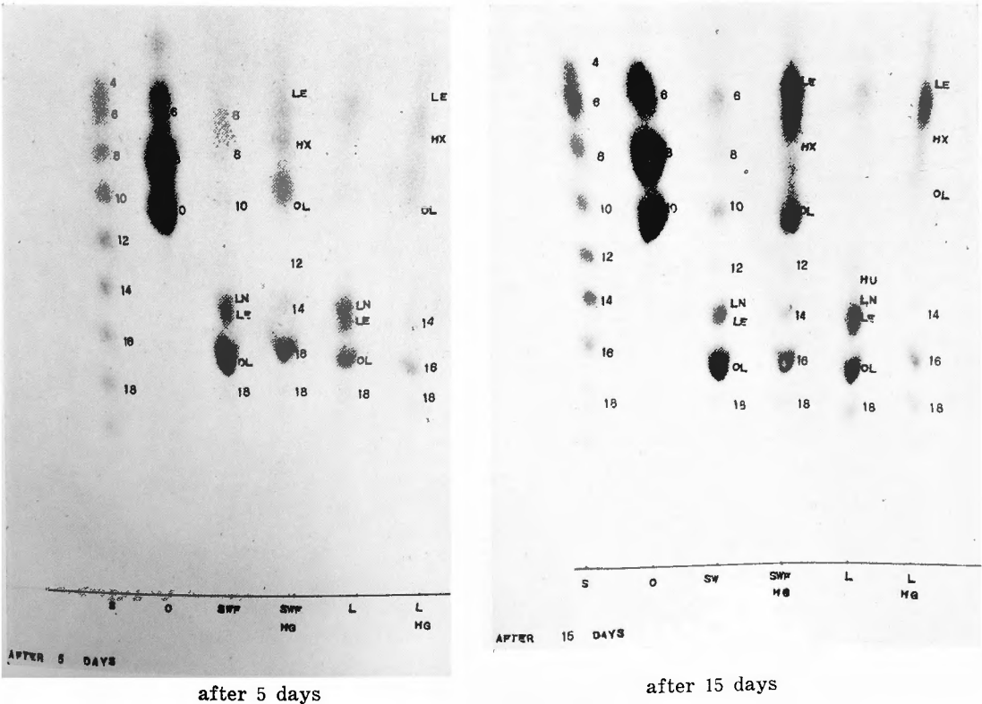
Fig. 12 Chromatogram of fatty acid in depot fat and liver in lower fatty acids diet group
