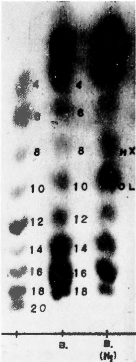
Fig. 4 Chromatogram of fatty acid in various adipose tissues and liver in low-fat diet group
