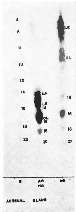
Fig. 17 Chromatogram of fatty acid in adrenal gland of normal dog
