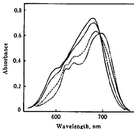
Fig. 2 \text{CoBr}_2 in acetone at high pressure and 25^\circ\text{C} Conc.: 1.856 \times 10^{-3} \text{ mol/l} Path length: 0.959 cm —: 1 kg/cm 2 ---: 880 kg/cm 2 - - - : 2910 kg/cm 2 - · - · : 5630 kg/cm 2
