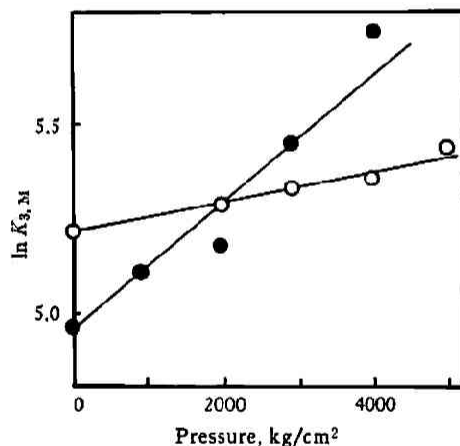
Fig. 11 Pressure dependence of K_3 , M at 25°C
