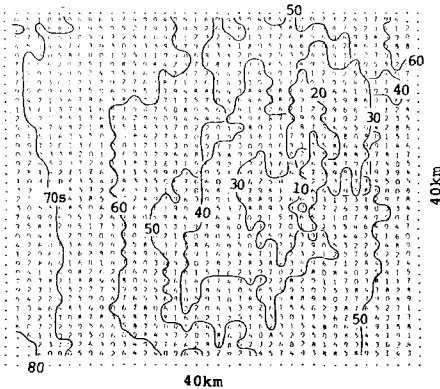
Figure 8. Patterns of rupture propagation for different B -values. (a) Case A, (b) Case B, (c) Case C.
