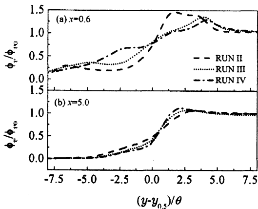
Fig. 3 Vertical distributions of time-averaged particle volume fraction. (a) x=0.6 , (b) x=5.0
