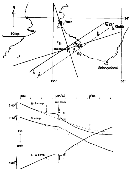
Fig. 1 Upper : Vector diagrams of anomalous tiltings observed about 4 months before the Shirahama-Oki Earthquake at Yura and Kishu
