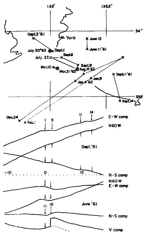
Fig. 3 Upper : Distribution of epicenters (Ref. Tables). The lines connecting two or more epicenters show a group of earthquakes Lower : Typical variations of ground-strain accompanied with a couple of earthquakes
