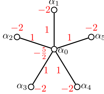
Figure 1. Dynkin diagram
