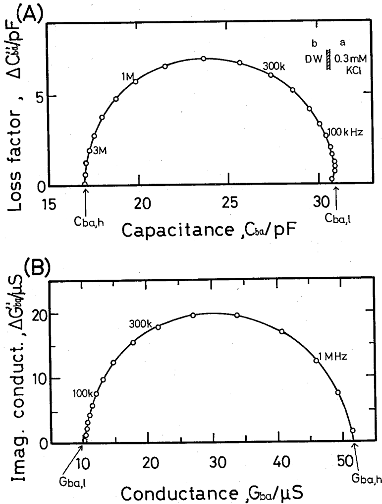
Fig. 11. Complex plane plots of (A) the complex capacitance C_{ba}^* [C_{ba}, \Delta C'' = (G_{ba} - G_{ba,l})/(2\pi f)] and (B) the complex conductance G_{ba}^* [G_{ba}, \Delta G'' = 2\pi f(C_{ba} - C_{ba,l})] for the composite Phase ba composed of Phase b (DW) and Phase a (0.3 mM KCl). The data referring to Fig. 10.
