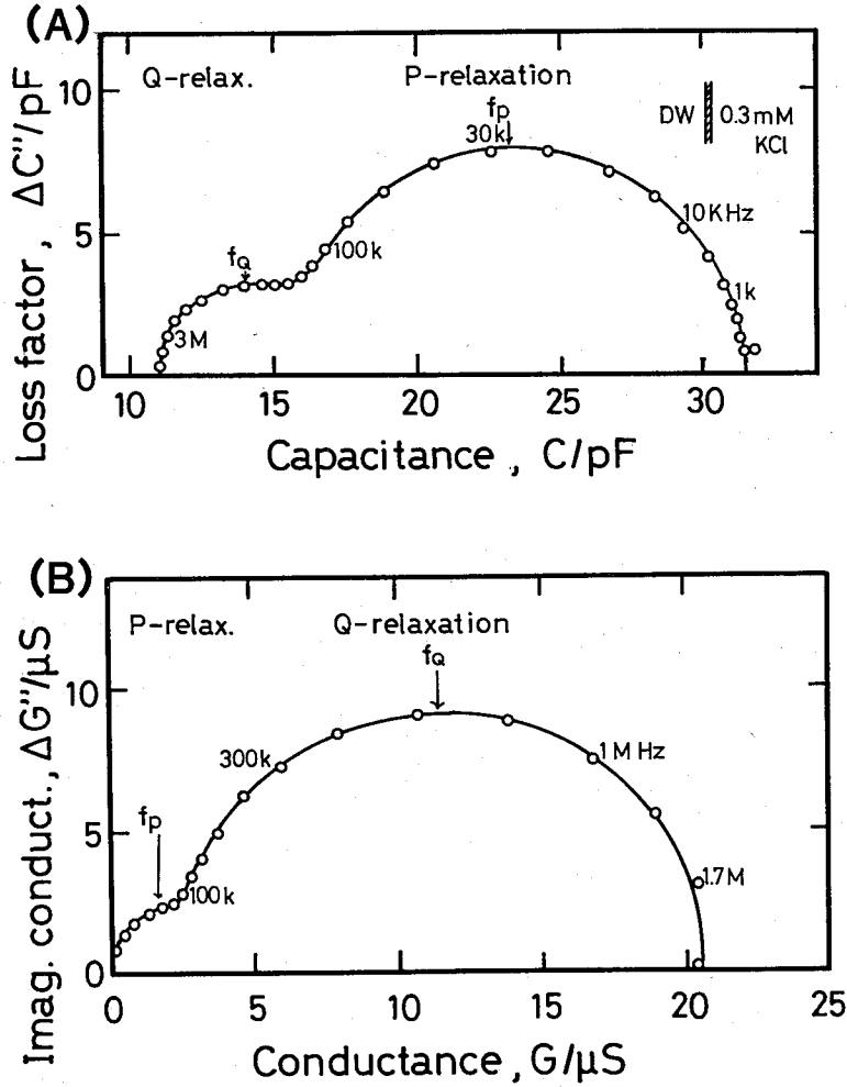
Fig. 7. Complex plane plots of (A) the complex capacitance C^* [ C , \Delta C'' = (G - G_0)/(2\pi f) ] and (B) the complex conductance G^* [ G , \Delta G'' = 2\pi f(C - C_0) ] for the whole system composed of DW-Teflon film-0.3 mM KCl. The data referring to the part of Fig. 6.
