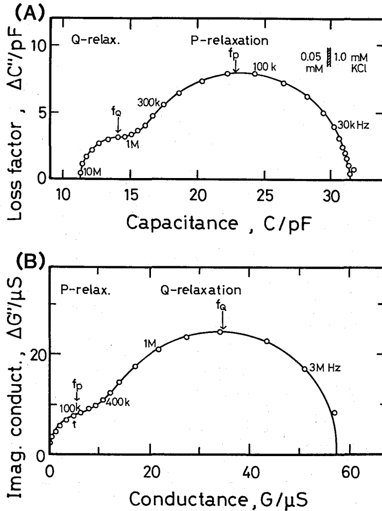
Fig. 9. Complex plane plots of (A) the complex capacitance C^* [ C, \Delta C'' = (G - G_l)/(2\pi f) ] and (B) the complex conductance G^* [ G, \Delta G'' = 2\pi f(C - C_h) ] for the whole system composed of 0.05 mM-Teflon film-1 mM KCl. The data referring to the part of Fig. 8.
