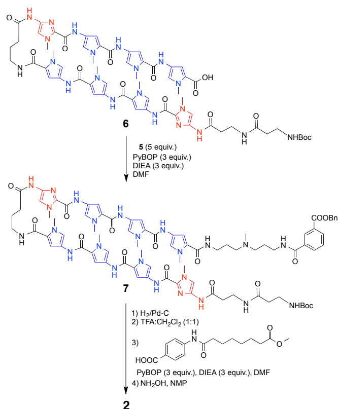
Scheme 2. Design and synthesis of isophthalic acid (IPA) conjugated SAHA-PIP 2
