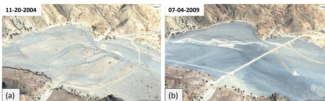
Fig. 11 Wadi channel morphology changes after Gonu cyclone in 2007. The sedimentation bars in Photo (a) were disappeared after the extreme floods (b) revealing to the huge transported sediment and the different in the soil colors is observed.
