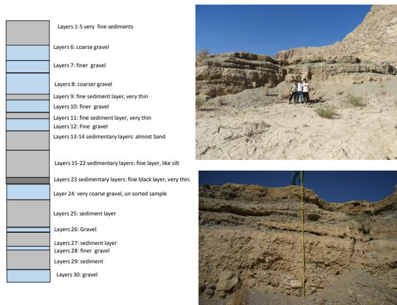
Fig. 12 Deposited sediments and layers were detected for analysis for paleo-flash floods ( Photos taken by Kyoto University Team, Field Survey on Nov. 29-Dec. 2, 2017 )
