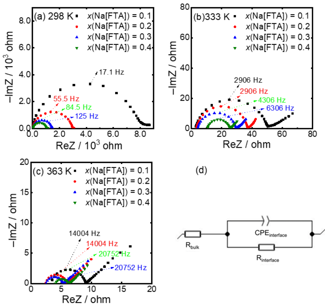
Figure 4-8. Nyquist plots of the Na/Na symmetric cells with the Na[FTA]-[C 3 C 1 pyrr][FTA] ILs ( x(\text{Na[FTA]}) = 0.1\text{--}0.4 ) at (a) 298 K (characteristic frequencies are 17.1 Hz for x(\text{Na[FTA]}) = 0.1 , 55.5 Hz for x(\text{Na[FTA]}) = 0.2 , 84.5 Hz for x(\text{Na[FTA]}) = 0.3 , 125 Hz for x(\text{Na[FTA]}) = 0.4 ), (b) 333 K (characteristic frequencies are 2906 Hz for x(\text{Na[FTA]}) = 0.1 , 2906 Hz for x(\text{Na[FTA]}) = 0.2 , 4306 Hz for x(\text{Na[FTA]}) = 0.3 , 6306 Hz for x(\text{Na[FTA]}) = 0.4 ), and (c) 363 K (characteristic frequencies are 14004 Hz for x(\text{Na[FTA]}) = 0.1 , 14004 Hz for x(\text{Na[FTA]}) = 0.2 , 20752 Hz for x(\text{Na[FTA]}) = 0.3 , 20752 Hz for x(\text{Na[FTA]}) = 0.4 ), in the frequency range of 100 kHz–10 mHz. (d) Equivalent circuit. AC amplitude = 10 mV.
