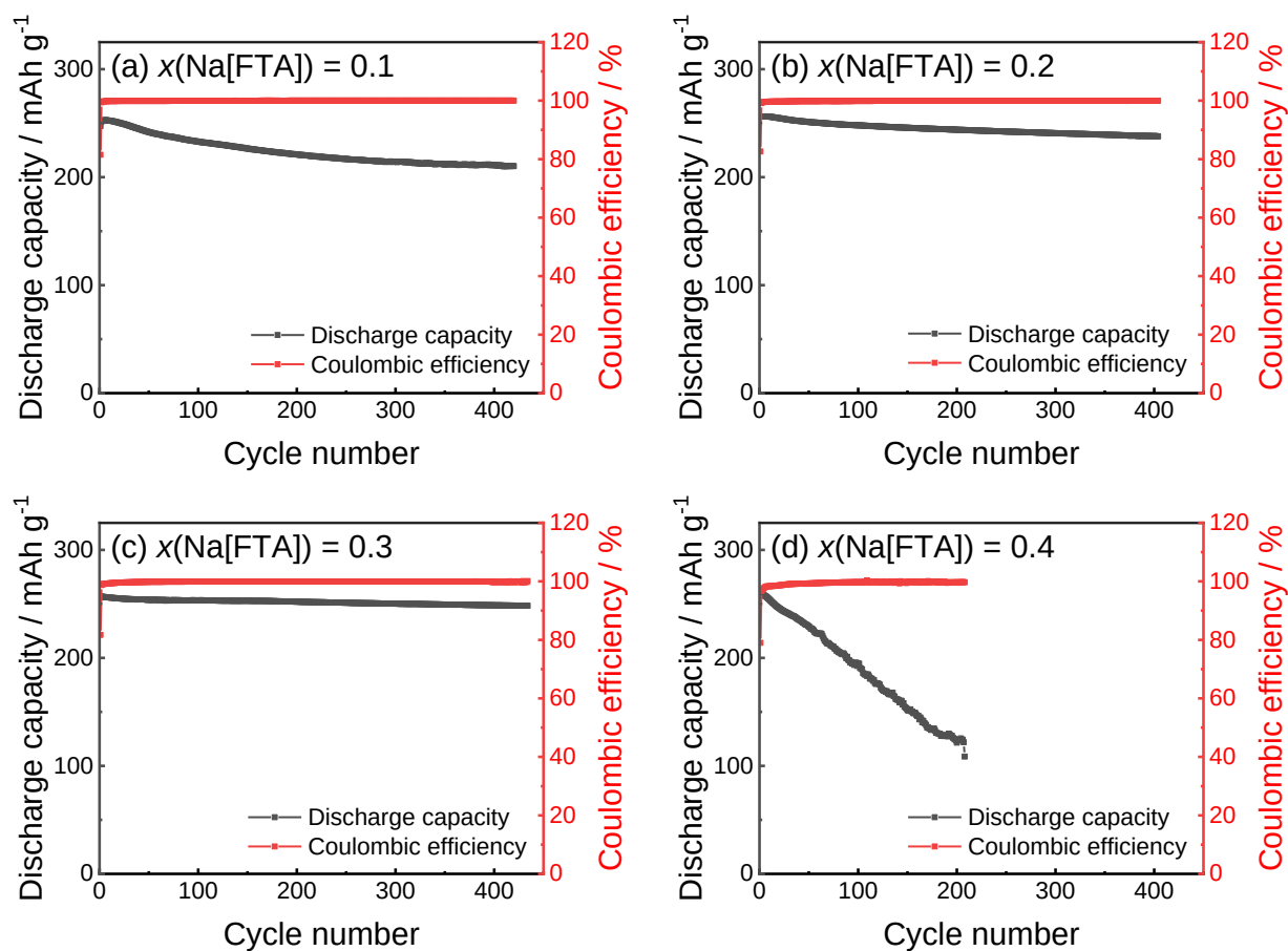
Figure 4-14. Cycling performance of the HC electrode at 363 K. Electrolyte: Na[FTA]-[C 3 C 1 pyrr][FTA] with x(\text{Na[FTA]}) = (a) 0.1, (b) 0.2, (c) 0.3, and (d) 0.4. Current rate: 200 mA g -1 . Cut-off voltages: 0.005–1.5 V.
