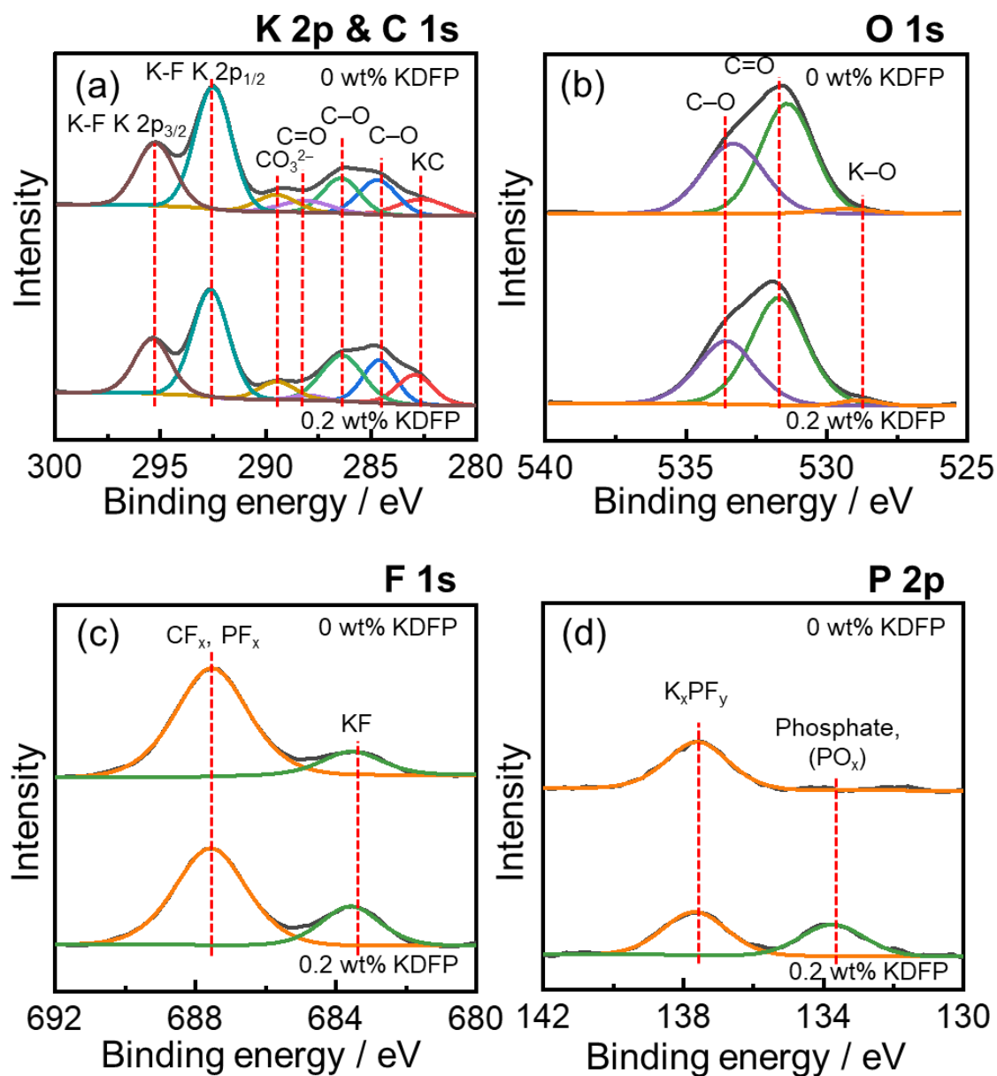
Figure 5-17. X-ray photoelectron spectra of SEI layers formed on graphite electrodes after 400 cycles in 0.5 M KPF 6 EC/DEC with and without KDFP additive in the (a) K 2p and C 1s, (b) O 1s, (c) F 1s, and (d) P 2p regions. The graphite electrodes after 400 cycles for XPS is in the fully depotassiation state. (See Table 5-4 for the binding energy of the peaks and SEI components)
