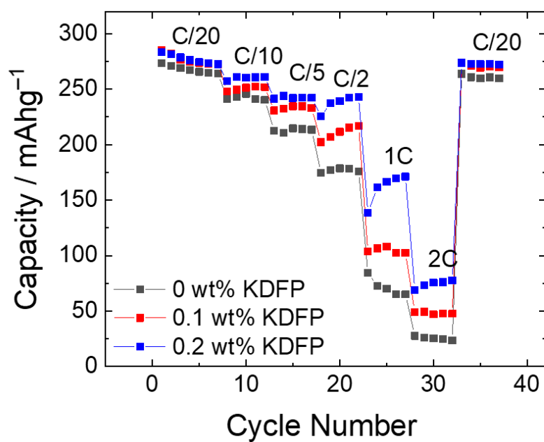
Figure 5-14. Rate capability of the K/graphite cells with 0.5 M \text{KPF}_6 -EC/DEC electrolytes containing different amounts of KDFP at 298 K. Rate: C/20 to 2C. Cut-off voltages: 0.001–2.5 V.
