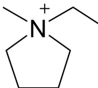
Figure 1-4 Structure of N -ethyl- N -methylpyrrolidinium cation ( \text{C}_2\text{C}_1\text{pyrr}^+ ).
