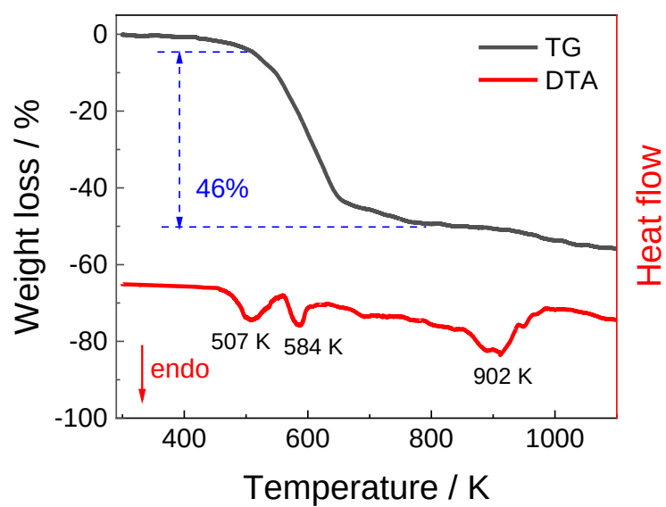
Figure 7-5. The TG-DTA curves of as-synthesized NaDFP. Scan rate: 1 K min -1 .
