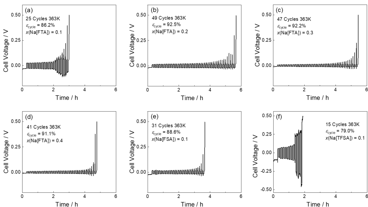
Figure 4-9. Voltage profiles during Na deposition/dissolution at 363 K in (a–d) Na[FTA]-[C 3 C 1 pyrr][FTA] at x(\text{Na[FTA]}) = 0.1\text{--}0.4 , (e) Na[FSA]-[C 3 C 1 pyrr][FSA] at x(\text{Na[FSA]}) = 0.1 , and (f) Na[TFSA]-[C 3 C 1 pyrr][TFSA] at x(\text{Na[TFSA]}) = 0.1 . The working and counter electrodes were Al and Na plates, respectively. Na metal of 0.08 \text{ C cm}^{-2} was deposited on the Al substrate, and 0.02 \text{ C cm}^{-2} Na deposition and dissolution was repeated until the electrode potential reached 0.5 V vs. Na + /Na during dissolution. The current density was \pm 0.1 \text{ mA cm}^{-2} for all tests.
