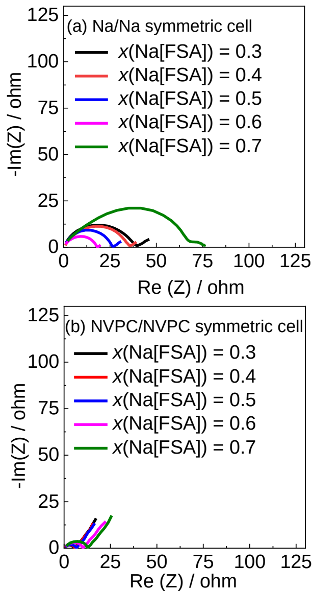
Figure 3-21. Nyquist plots of (a) the Na/Na symmetric and (b) NVPC/NVPC symmetric (SOC = 0.5) cells in Na[FSA]–[C 2 C 1 pyrr][FSA] ( x(\text{Na[FSA]}) = 0.3\text{--}0.7 ) at 363 K (1 d after cell assembling). AC perturbation: 10 mV, frequency range: 10 mHz to 100 kHz. R_b is set as zero to compare R_{ct} in all the plots.
