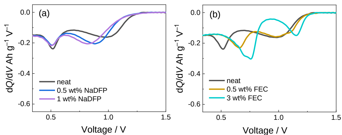
Figure 6-6. The dQ/dV plots of the first charge curve in (a) 1 M \text{NaPF}_6 -EC/DMC (1:1, v:v) with 0 wt% additive (neat), 0.5 wt% NaDFP, and 1 wt% NaDFP, (b) 1 M \text{NaPF}_6 -EC/DMC (1:1, v:v) with 0 wt% additive (neat), 0.5 wt% FEC, and 3 wt% FEC.
