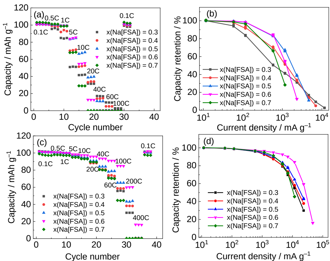
Figure 3-15. Rate capability of the Na/NVPC cells at (a, b) 298 K and (c, d) 363 K. Electrolyte: Na[FSA]–[C 2 C 1 pyrr][FSA] ( x(\text{Na[FSA]}) = 0.3\text{--}0.7 ). Charge rate: 0.1C, discharge rates: 0.1C–400C, cut-off voltages: 2.4–3.8 V.
