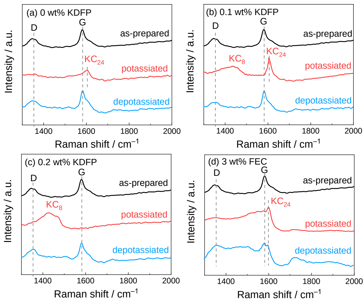
Figure 5-12. Raman spectra of graphite electrodes at pristine (black), fully potassiated (red), and fully depotassiated (blue) states. Electrolytes: 0.5 M \text{KPF}_6 -EC/DEC with (a) 0 wt% KDFP, (b) 0.1 wt% KDFP, (c) 0.2 wt% KDFP, and (d) 3 wt% FEC.
