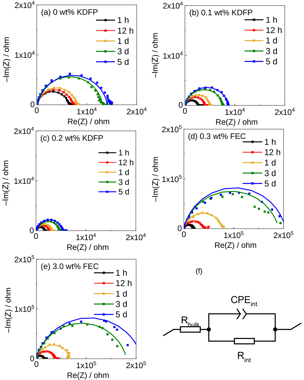
Figure 5-7. Nyquist plots and fitting lines of the K/K symmetric cells at 298 K using the 0.5 M KPF 6 -EC/DEC electrolyte with (a) 0 wt% KDFP, (b) 0.1 wt% KDFP, (c) 0.2 wt% KDFP, (d) 0.3 wt% FEC, and (e) 3 wt% FEC in the frequency range of 100 kHz–10 mHz. (f) Equivalent circuit used for data fitting. AC amplitude: 10 mV.
