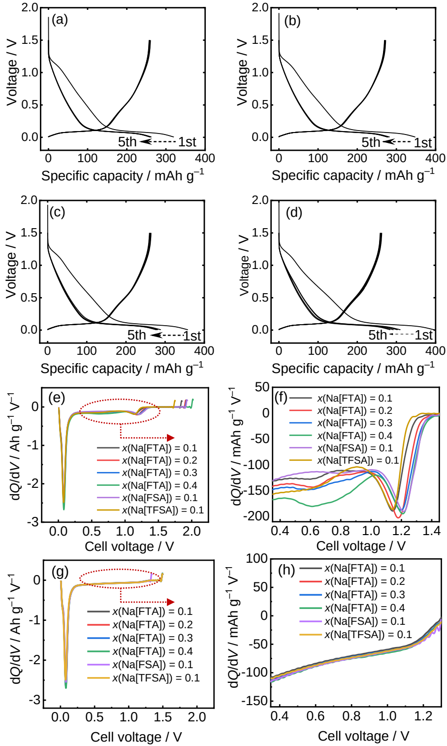
Figure 4-10. Charge-discharge curves of the Na/HC cells with the Na[FTA]-[C 3 C 1 pyrr][FTA] ILs at x(\text{Na[FTA]}) = (a) 0.1, (b) 0.2, (c) 0.3, and (d) 0.4 at 363 K. Charge-discharge rate: 20 mA g -1 . The corresponding differential capacity vs. voltage ( dQ/dV ) plots (e, f) and (g, h) show the first and fifth charge cycle behavior with those observed for Na[FTA]-[C 3 C 1 pyrr][FTA] ILs at x(\text{Na[FTA]}) = 0.1-0.4 , Na[FSA]-[C 3 C 1 pyrr][FSA] at x(\text{Na[FSA]}) = 0.1 and Na[TFSA]-[C 3 C 1 pyrr][TFSA] at x(\text{Na[TFSA]}) = 0.1 .
