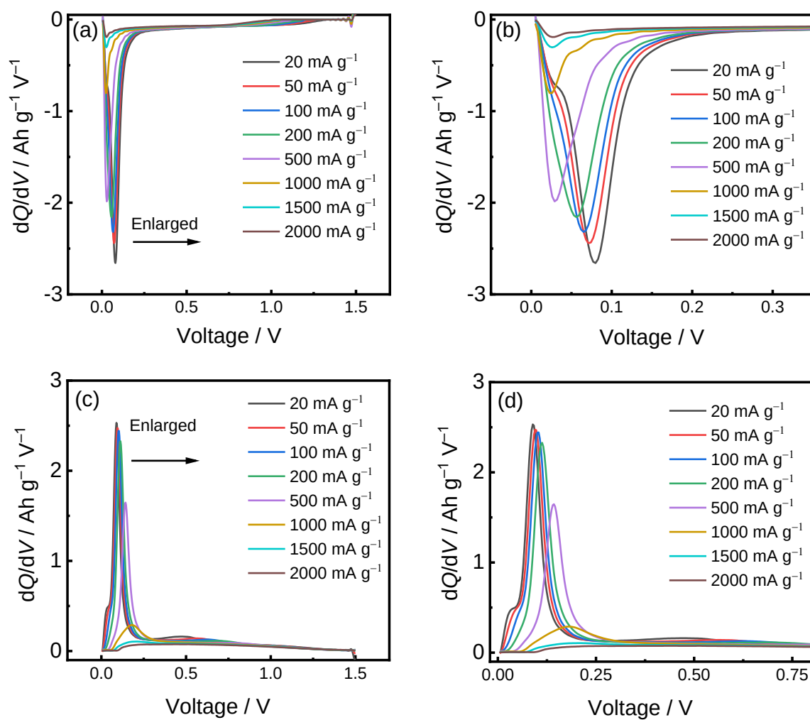
Figure 4-13. The dQ/dV plots of (a, b) charge and (c, d) discharge curves of the HC/Na cell with the Na[FTA]-[C 3 C 1 pyrr][FTA] IL at x(\text{Na[FTA]}) = 0.3 in charge-discharge rate from 20 to 2000 mA g -1 at 363 K.
