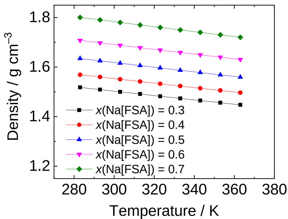
Figure 3-7. Temperature dependence of Na[FSA]-[C 2 C 1 pyrr][FSA] density at x(\text{Na}[\text{FSA}]) = 0.30\text{--}0.70 .
