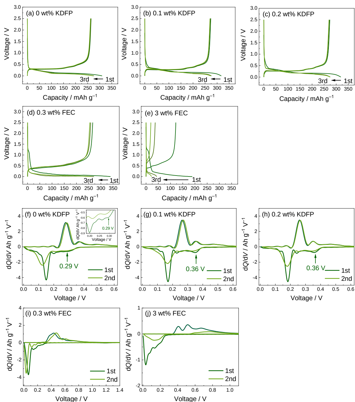
Figure 5-9. Charge-discharge curves of the K/graphite cells in 0.5 M \text{KPF}_6\text{-EC/DEC} with (a, f) 0 wt% KDFP, (b, g) 0.1 wt% KDFP, (c, h) 0.2 wt% KDFP, (d, i) 0.3 wt% FEC, and (e, j) 3 wt% FEC. Current density: C/20 ( 1\text{C} = 279 \text{ mA g}^{-1} ). The corresponding differential capacity vs. voltage ( dQ/dV ) plots of the first two charge-discharge cycles are shown in (f–j). (See Table 5-2 for the peak position during potassiation and depotassiation of the initial cycle.)
