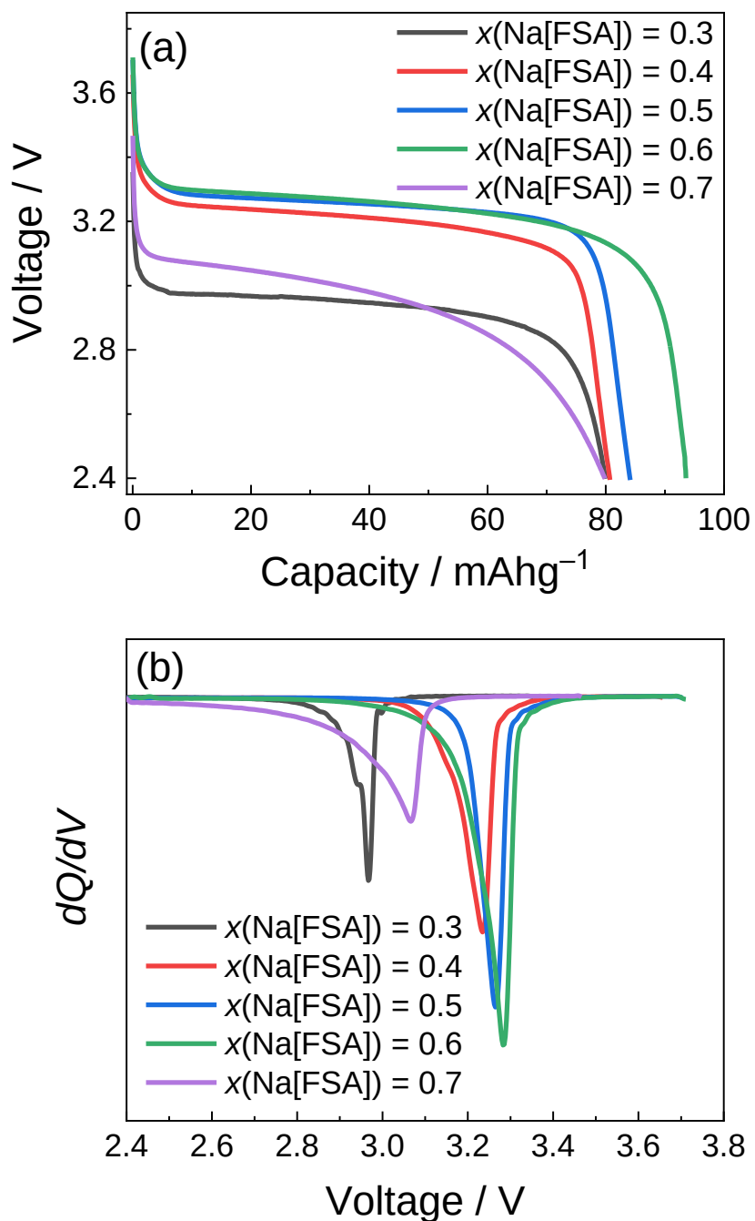
Figure 3-17. (a) The discharge curves of Na/NVPC cells at 363 K operated at 40C and (b) the corresponding ( dQ/dV ) plot. Electrolyte: Na[FSA]–[C 2 C 1 pyrr][FSA] ( x(\text{Na}[\text{FSA}]) = 0.3\text{--}0.7 ).
