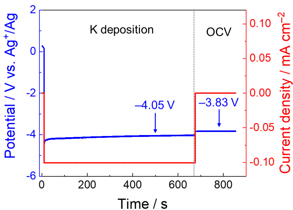
Figure 5-2. The voltage profile of K deposition/dissolution in 0.5 M KPF 6 -EC/DEC on the Al working electrode (area: 0.25 cm 2 ) with the Ag + /Ag reference electrode and Pt counter electrode in a three-electrode cell. The K + /K equilibrium potential in 0.5 M KPF 6 -EC/DEC is determined to be -3.83 V vs. Ag + /Ag by an open circuit potential (OCP) measurement after galvanostatic K metal deposition at 0.1 mA cm -2 in a three-electrode cell.
