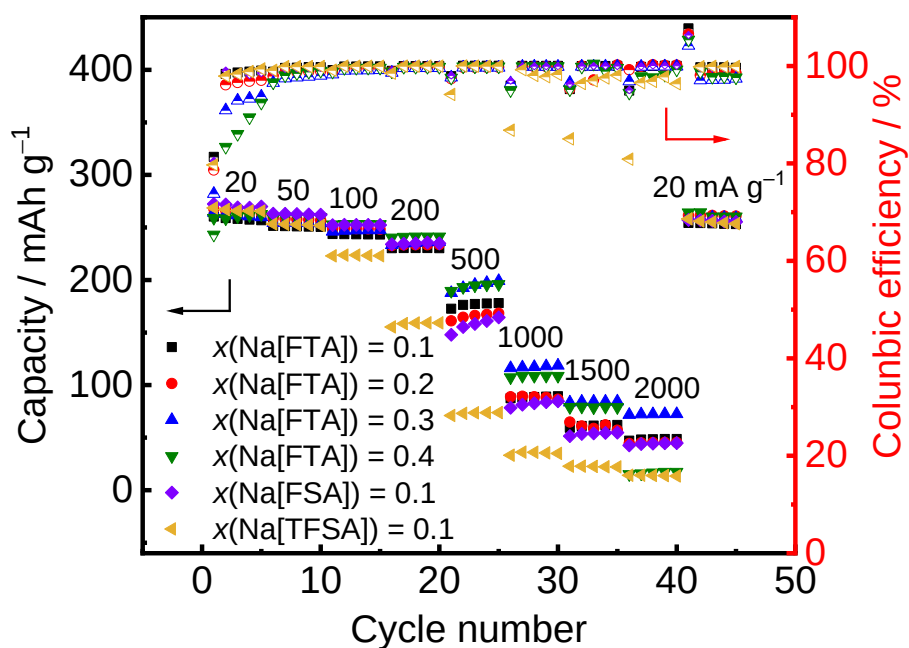
Figure 4-11. Rate capability of the Na/HC cells with Na[FTA]-[C 3 C 1 pyrr][FTA] at x(\text{Na[FTA]}) = 0.1 – 0.4 , Na[FSA]-[C 3 C 1 pyrr][FSA] at x(\text{Na[FSA]}) = 0.1 , and Na[TFSA]-[C 3 C 1 pyrr][TFSA] at x(\text{Na[TFSA]}) = 0.1 at 363 K. Charge-discharge rate: from 20 to 2000 \text{mA g}^{-1} . Cut-off voltages: 0.005–1.5 V. Coulombic efficiency is plotted with half-filled marks.
