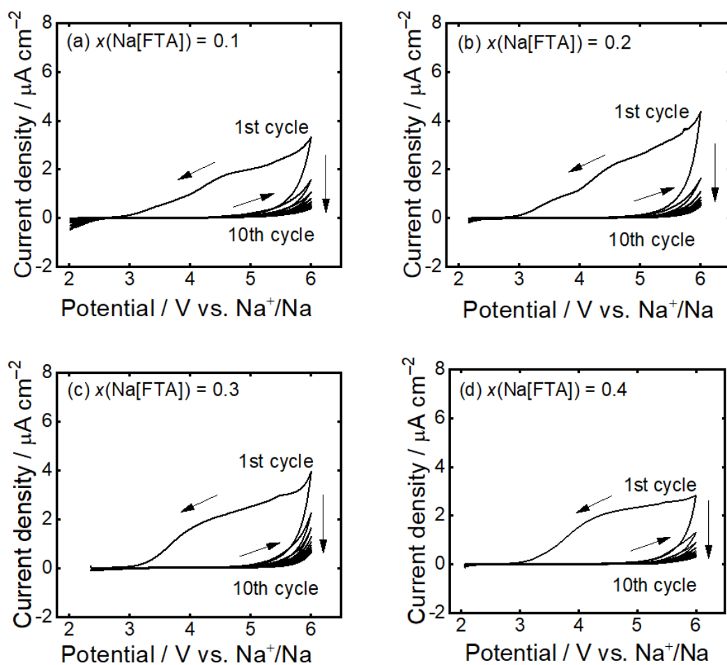
Figure 4-6. Cyclic voltammograms of an Al electrode at 298 K in the Na[FTA]-[C 3 C 1 pyrr][FTA] ILs at x(\text{Na[FTA]}) = (a) 0.1, (b) 0.2, (c) 0.3, and (d) 0.4 recorded at a scan rate of 1 mV s -1 .
