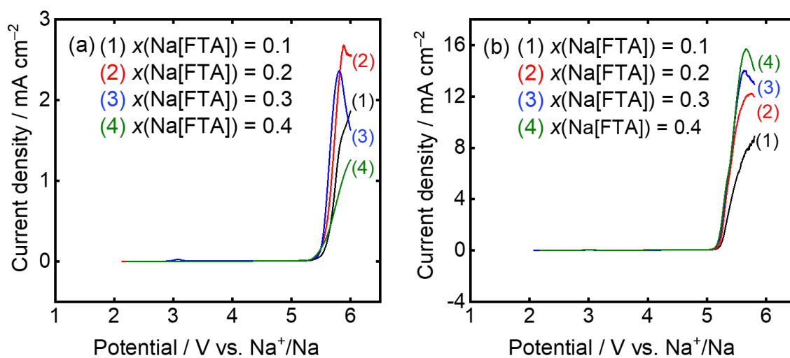
Figure 4-5. Linear sweep voltammograms of a Pt electrode at a scan rate of 1 \text{ mV s}^{-1} in the Na[FTA]-[C 3 C 1 pyrr][FTA] ILs at x(\text{Na[FTA]}) = 0.1\text{--}0.4 at (a) 298 K and (b) 363 K.
