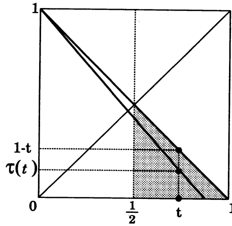
Figure 7: Case 2-2 ( a_r < 0 , t \geq \frac{1}{2} , and \tau(t) \leq 1 - t )
