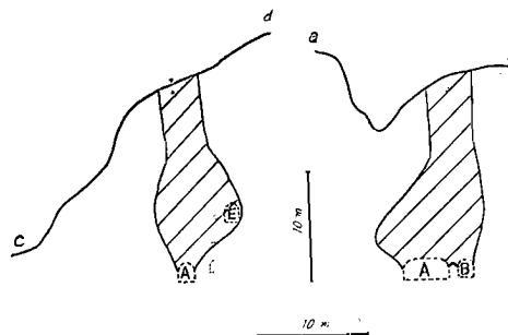
Fig. 7. Vertical sections a-b and c-d on the part of rock-falling. A : -New drift, B : -Old drift, E : -Dead drift
