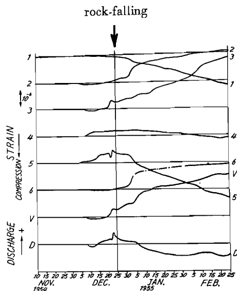
Fig. 8. Variations of ground-strain and discharge of mine water before and after the occurrence of rock-falling.
