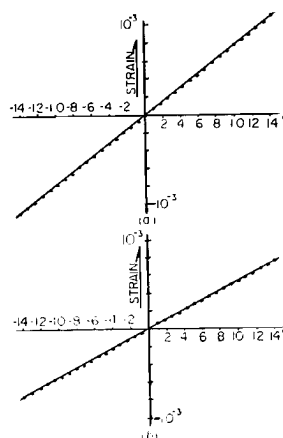
Fig. 21. Sensitivity of the portable underground inclinometer. (Relation between the angle of inclination and strain)
