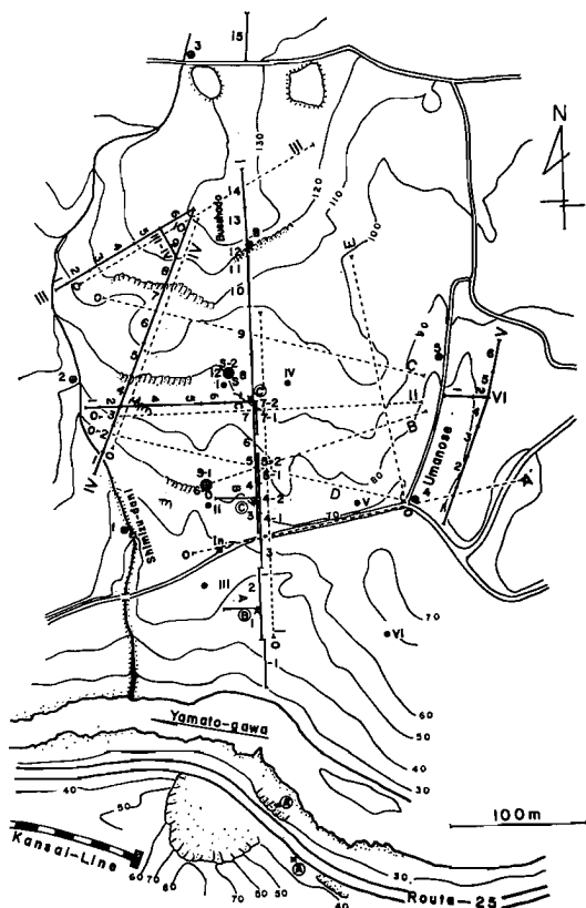
Fig. 16. Disposition and distribution of the instruments and traverse lines of seismic prospecting. I : -1, 1, 2, .....15, II : 1, 2, ---7 (=c), III : 1, 2, ---6, IV : 1, 2, ---10, V : 1, 2, ---6, VI : 1, 2, III-IV, A, B, S : Extensometer, \times : (A), (A'), (B), (C), (C') : Tiltmeter, \oplus : 1, ---5, 6, 12 : -Observing well of groundwater level, \bullet : 1, II, ---, B : -Travelling post, In : -Portable underground inclinometer, \oplus S-1 : -Shaft-No. 1, \oplus S-2 : -Shaft-No. 2, --- : -Traverse line of seismic prospecting
