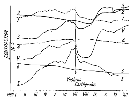
Fig. 3. Variations of linear strains and volume dilatation of which eliminated annual variations and variations caused by rainfall at Ide.
