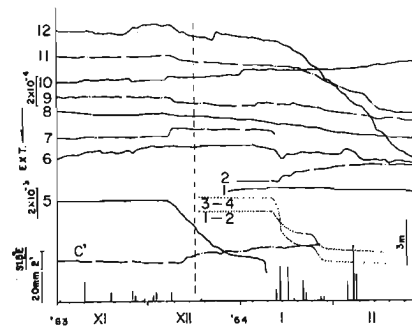
Fig. 25. Variations of ground-strain and ground-tilt before and after the crack-occurrence and the precipitation.
