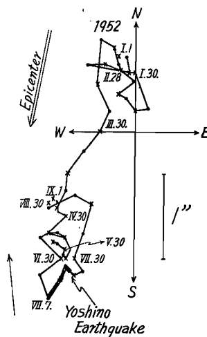
Fig. 5. Variation of ground-tilt observed at the Osakayama Observatory (by Prof. I. Ozawa).
